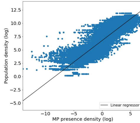
FIGURE 4.11: Linear regression between mobile phone presence at 03 AM and population densities for census blocks at logarithmic scale.
