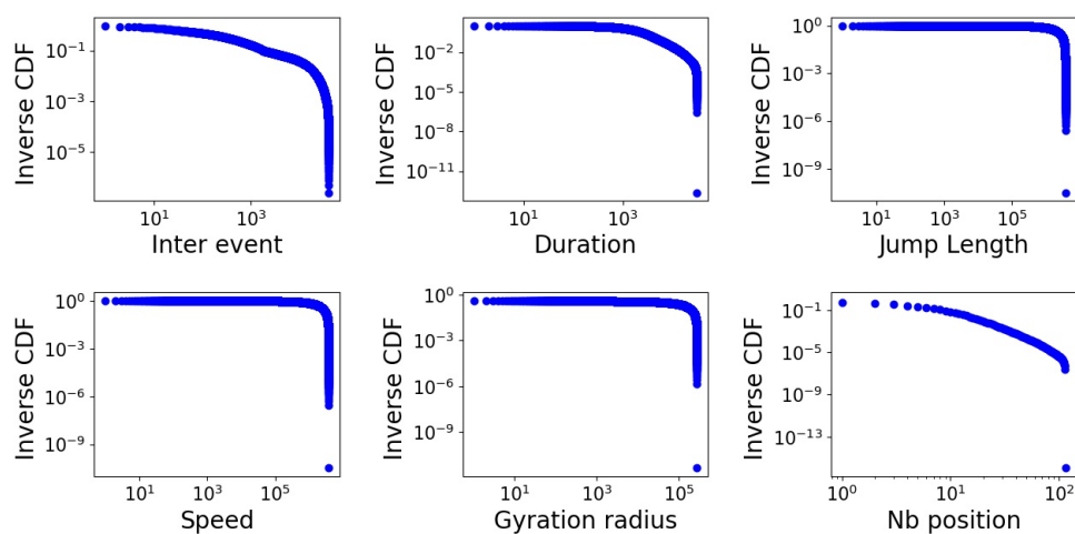
FIGURE 3.6: Inverse Cumulative Distributions of Trajectory attributes
