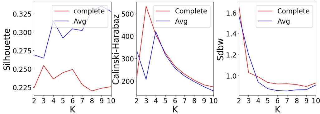
FIGURE 4.4: Clustering evaluation metrics for the standard scaler normalization, correlation distance and hierarchical clustering.
