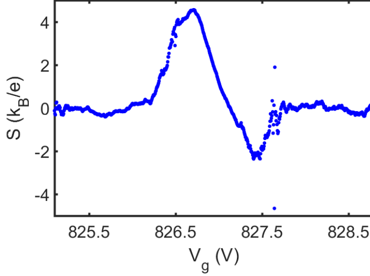
Fig. 5.14: Gate voltage dependence of the thermopower Thermopower S of the QD junction is plotted with the gate voltage, measured at a bath temperature T_b = 70 \text{ mK} . It is extracted from the thermovoltage data, normalized with the temperature difference \Delta T = 92 \text{ mK} between the source and drain lead, determined by the fitting of thermocurrent data with linear response theory as described before.
