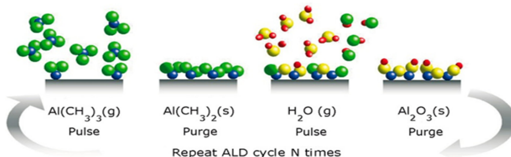
Fig. 2.2: Steps of a single ALD cycle (Adapted from Oxford instruments) Schematic diagram of the steps of a single layer of \text{Al}_2\text{O}_3 deposition on top a substrate using ALD technique. First, the precursor of \text{Al}_2\text{O}_3 TMA is injected in to the chamber, after the completion of the reaction the product is removed from the chamber with the purge of dry \text{N}_2 , next the precursor \text{H}_2\text{O} is injected and in the same way products are purged out of the chamber and in this way a single layer of \text{Al}_2\text{O}_3 is deposited on top of the substrate. A single cycle produces approximately 1 nm thick \text{Al}_2\text{O}_3 layer, N cycles are repeated to get a N nm thick layer of \text{Al}_2\text{O}_3
