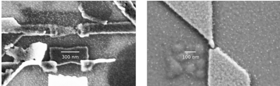
Fig. 2.9: NPs deposited by drop-cast method SEM image for the distribution of 5 nm Au – NPs deposited on top of the electromigrated junction, deposited by the drop cast method. The yield of this method for a successful QD device is about 3%.
