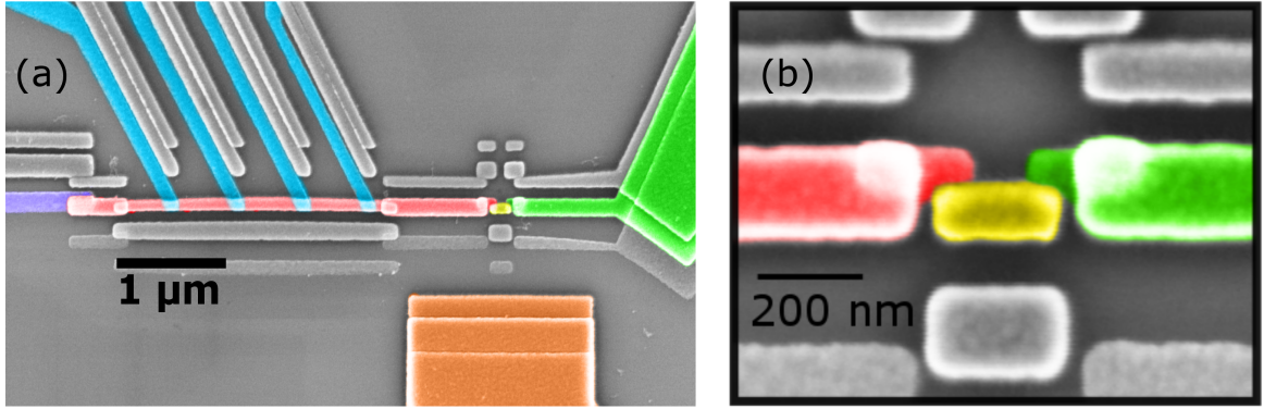
Fig. 2.3: SEM image of the SET device (a) Colored SEM image of the SET with different elements of the device shown in different color: the Source is shown in red, Clean-contacted Al lead at the end of source in purple, four tunnel-contacted Al leads in cyan, the Island in yellow, the Drain in Green and the Gate is shown in orange color. (b) Zoomed in view of the SET, showing two Al dots connected to the island via tunnel contact (in red and green on the left and right of the island), while on the opposite side they are connected to big metallic Cu strips, in order to destroy the SC of the Al dots
