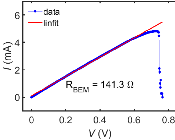
Fig. 2.7: IV curve of a typical EM A typical IV curve for an EM process. The resistance of the constriction before EM is measured to be R_{\text{BEM}} = 141 \, \Omega . The EM process stops as soon as the measured conductance of the junction drops below a preset value.
