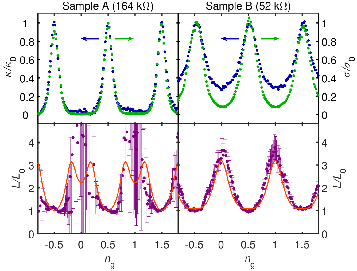
Fig. 4.8: Comparison of charge and thermal conductance (Adapted from Dutta et al. [103])
