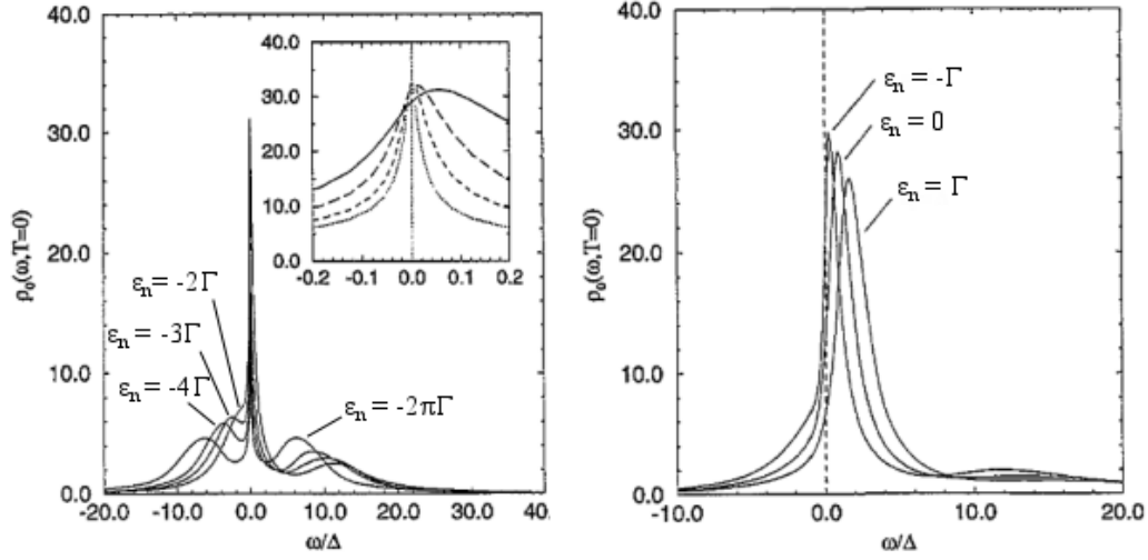
Fig. 1.8: Spectral function of a Kondo-correlated QD (Adapted from Costi et al. [35]) (a) spectral function of a Kondo-correlated QD at T = 0 , for symmetric level position, \epsilon_n/\Gamma = -2\pi and for three asymmetric level positions \epsilon_n/\Gamma = -4, -3, -2 , where Kondo resonance still persists. Inset shows that Kondo resonance is pinned to the Fermi level ( \omega = 0 ) for the symmetric case, while for asymmetric case Kondo-resonance is shifted slightly above Fermi energy with increasing asymmetry. (b) Spectral function at T = 0 , for a more asymmetric case where QD is in the mixed valence and empty orbital regime. Here the Kondo resonance is overcome by the Coulomb-peak.
