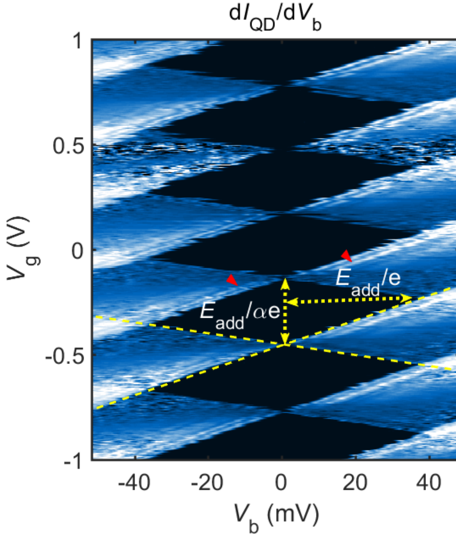
Fig. 5.2: long range stability diagram of the QD made of evaporated Au NP Conductance map of the QD in the bias and gate voltage plane. The Coulomb diamonds are identified as the black regions. Inside the conductive region some highly conductive bright lines can be observed, indicated by the red arrow-heads. These lines are the indication of quantization of energy of the QD . The extents of a diamond gives the amount of addition energy E_{add} needed to put an extra electron into the QD level.
