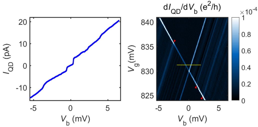
Fig. 5.10: Conductance map of the QD: Exp 2 (a) Current-Voltage characteristics of the QD junction along the yellow line shown in (b) at a fixed gate voltage V_g = 831.2 \text{ mV} , the step height for positive and negative currents allow us to estimate the two tunnel rates. (b) Stability diagram for differential conductance of the QD junction. The differential conductance is calculated from the measured I_{QD} vs V_b curves at different gate voltages. Due to the very high charging energy E_c (> 200 \text{ meV}) of the QD, only one charge degeneracy point is observed at V_g \approx 830 \text{ mV} , separating two charge states. The black contrast regions are the Coulomb blocked area. The bright lines separate the blocked region from the conductive region forming the Coulomb diamond edges. Inside the conductive region some bright lines (indicated by red arrow-head) are observed, these lines correspond to the quantized single levels of the QD. Beside these lines some other regularly spaced line structures can also be found in this conductive region, these could be attributed to the vibrational modes of the QD
