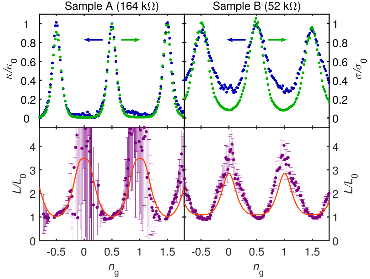
Fig. 4.9: Comparison of charge and thermal conductance in the heating regime Top: Thermal and electrical conductances of the SET for sample A (left) and sample B (right) at a bath temperature of 132 mK (sample A) and 152 mK (sample B). The thermal flow through the SET was calculated assuming that the Wiedemann-Franz law is fulfilled at gate-open state. The charge transport measurement was done at a bias of 22.4 \mu\text{V} (sample A) and 19.2 \mu\text{V} (sample B). The heat transport data was acquired by heating the source electronic bath by 60 mK (sample A) and 52 mK (sample B) above the bath temperature. Bottom: Lorenz ratio defined as L/L_0 where L = \kappa/(\sigma T_m) for sample A (left) and sample B (right). The red line is the theoretical prediction.
