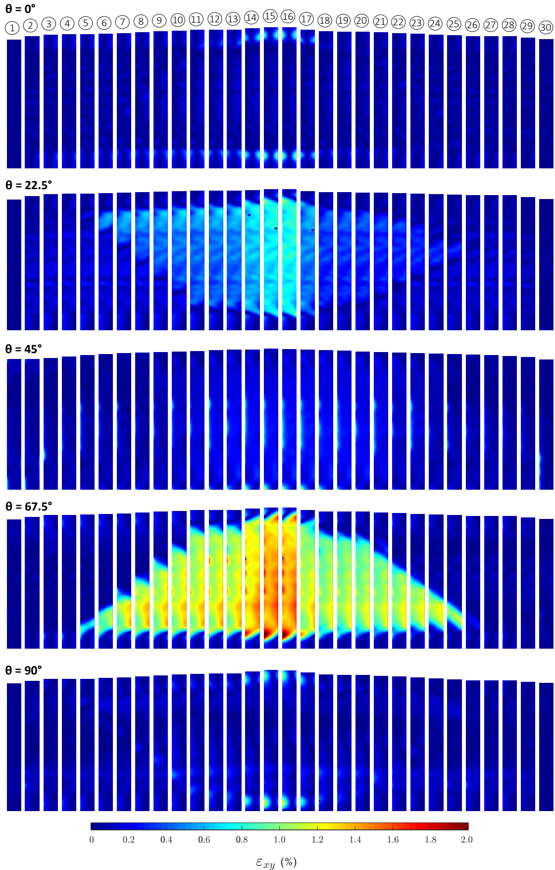
Figure 4.8: Shear strain maps ( \epsilon_{xy} ) of oriented samples under tensile load at 60^\circ\text{C} .
