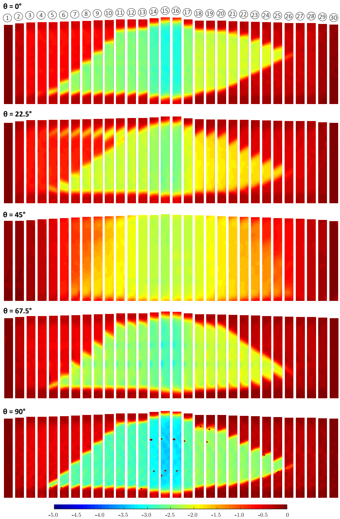
Figure B.2: Transverse strain maps ( \varepsilon_{xx} ) of oriented samples under tensile load at 40^\circ\text{C} .
