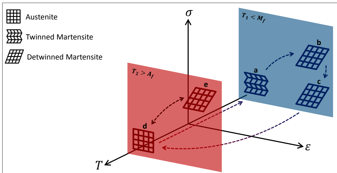
Figure 1.1: Temperature ( T ) - stress ( \sigma ) - strain ( \varepsilon ) space showing the regions where austenite and martensite phases are stable.
