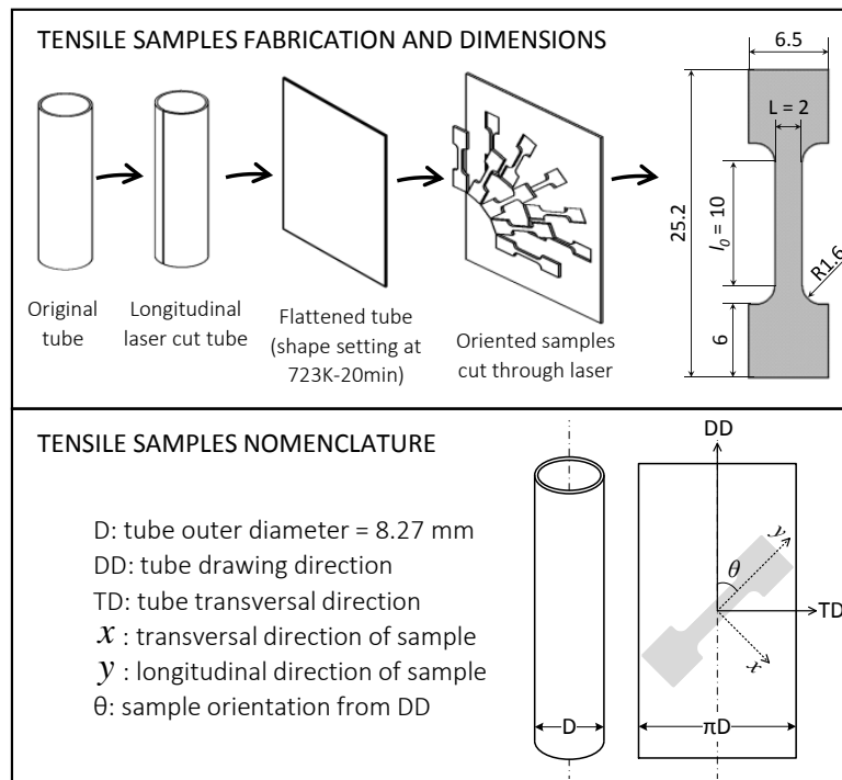
Figure 3.1: Scheme of fabrication process of dogbone tensile samples from NiTi tube, the final dimensions of samples and adopted nomenclature.
