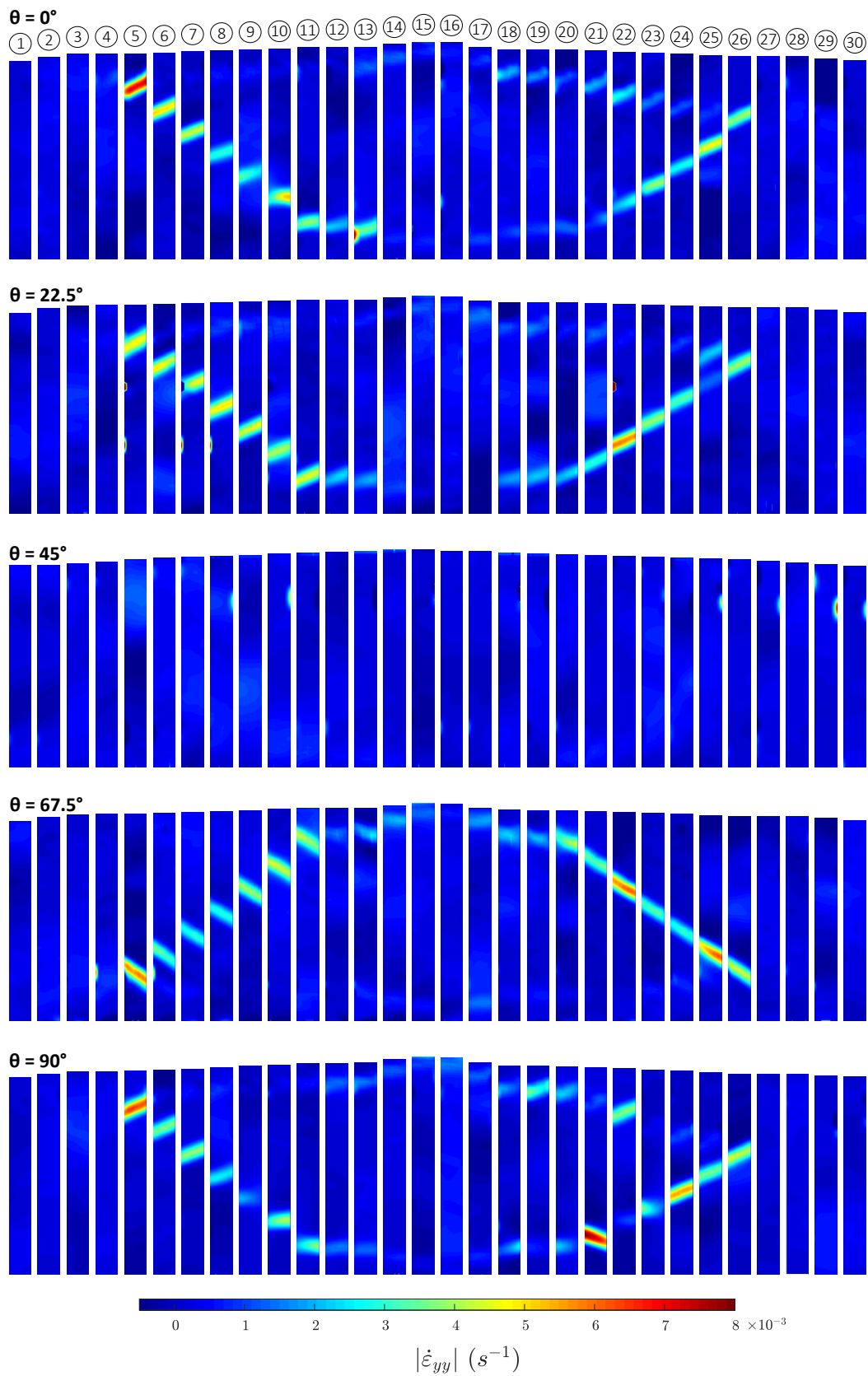
Figure B.10: Longitudinal strain rate maps ( |\dot{\epsilon}_{yy}| ) of oriented samples under tensile load at 50°C.
