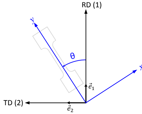
Figure 4.2: Tensile sample oriented in an arbitrary direction in the plane of the sheet metal. A new coordinate system is defined by an x -axis in its width direction and a y -axis in its longitudinal direction.
