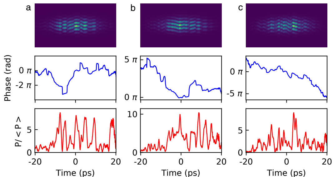
FIGURE 4.15: Experimentally recorded with HTM partially-coherent waves propagated in 900 m fiber with normal dispersion. Spectral width is 0.5 THz, average power is 4.5 W. (first row) snapshots recorded directly with the HTM. (second and third rows) reconstructed phase and power profiles.
