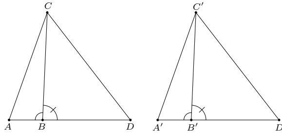
FIGURE I.2.7. Hilbert's Theorem 14.
