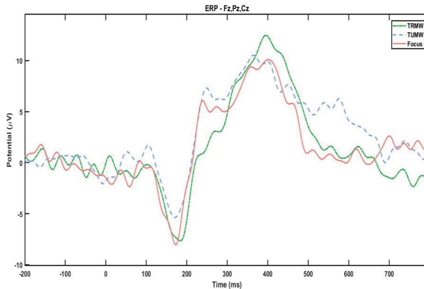
Figure 45. Beep ERP signal for each attentional state.
