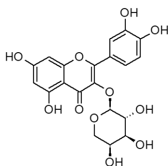
Guaijaverine
