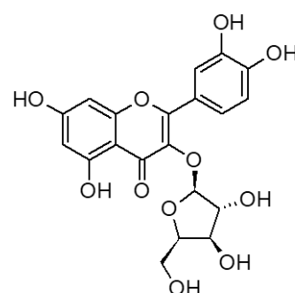
Quercitine-3-O-β-D-xylofuranoside
