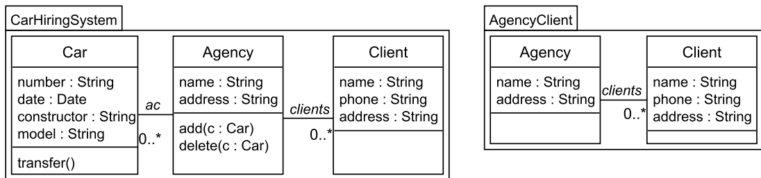
FIGURE 4.1 – AgencyClient et CarHiringSystem
