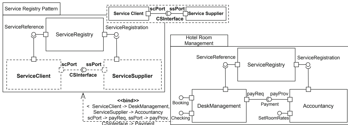
FIGURE 2.32 – Aspectual templates de composants (Source :Vanwormhoudt et al. [103])
