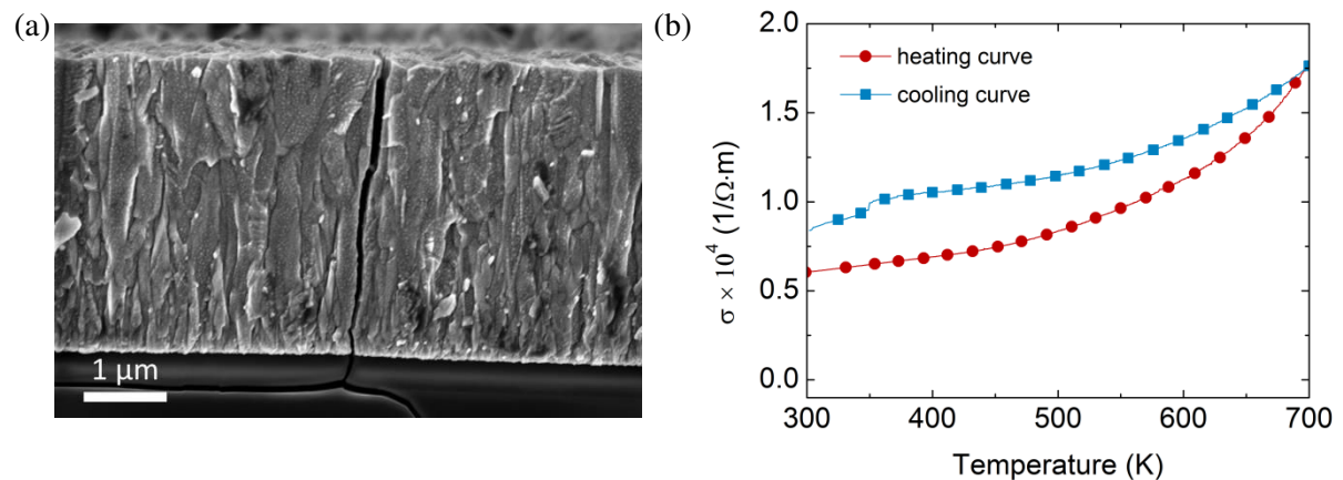
Figure 3.5. Mg 2 (Si,Sn) thin film deposited on SiO 2 /Si substrate at 463 K after TT (700 K): (a) cross-sectional SEM image and (b) electrical conductivity measurement.
