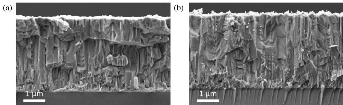
Figure 3.16. Cross-sectional SEM images of \text{Mg}_2(\text{Si},\text{Sn}) thin film deposited at 463 K on borosilicate glass substrate: (a) before and (b) after TT at 653 K for 168 h.
