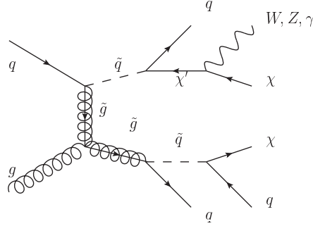
Figure 3.1: An example for strong production of a pair of supersymmetric particles (in this case, a squark and a gluino) which subsequently decay through a cascade, with a final state containing multiple quarks, possibly leptons and a higgsino pair.
