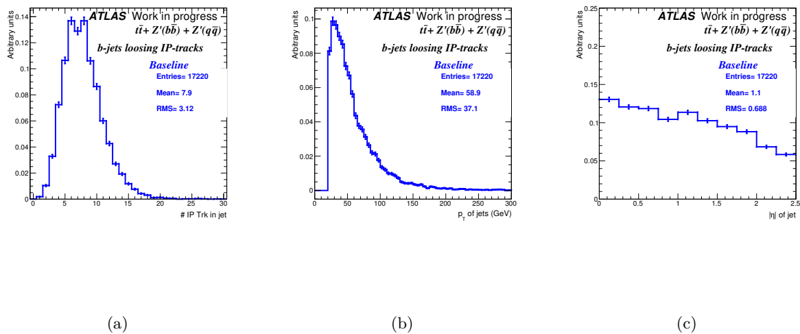
Figure 9.15.: (a) b-tagging quality track multiplicity, (b) p_T and (c) \eta distributions for b-jets losing tracks.
