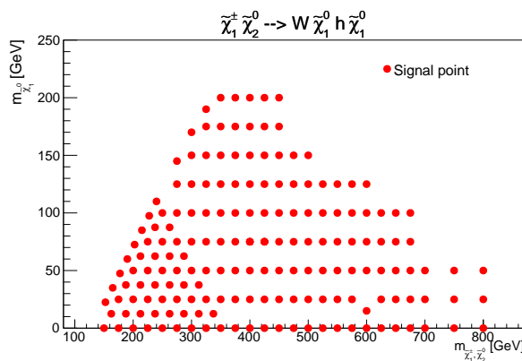
Figure 10.5.: The signal grid plotted in the (m_{\tilde{\chi}_1^\pm, \tilde{\chi}_2^0}, m_{\tilde{\chi}_1^0}) plane [99].
