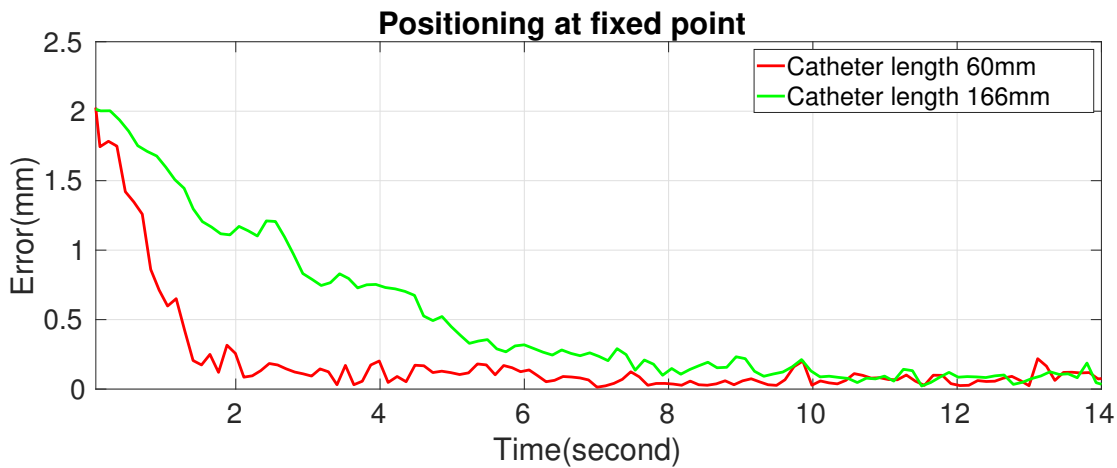
Figure 5.7: Convergence of positioning errors with different catheter length (60mm and 166mm).
