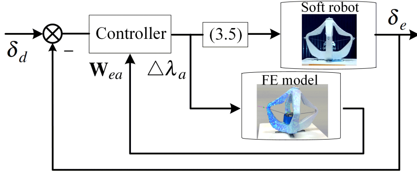
Figure 3.2: The first implementation of closed-loop control. Information from both the soft robot and the FE model is needed to compute the control inputs. The FE model provides the value of compliance matrix in (3.4) for the controller.
