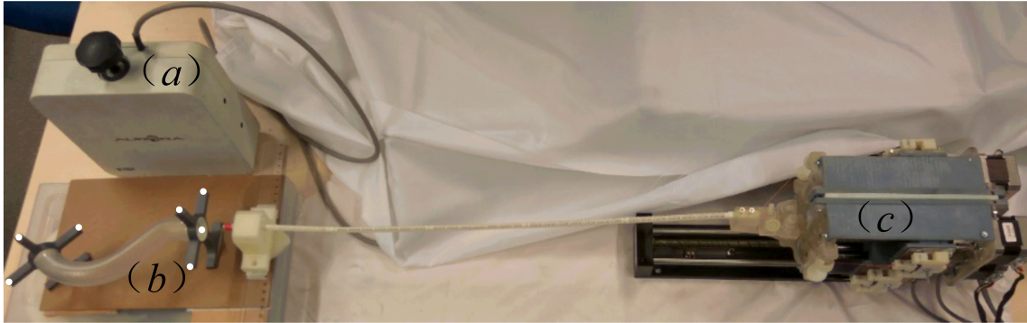
Figure 5.4: Experimental setup for the motion control of a catheter robot through contacts. (a) NDI electromagnetic tracking system: Aurora; (b) a rigid tube for the experiment. The white points are the feature points which are used for the calibration; (c) the cable-driven continuum catheter robot which has four step motors to actuate the bending and one step motor to control the insertion.
