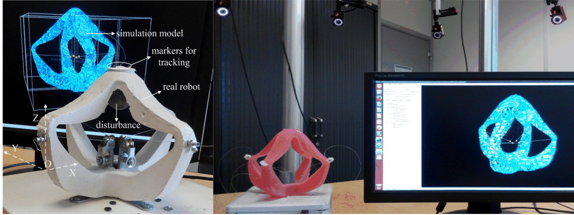
Figure 3.6: Experimental setup for the position control of soft robots. Two soft parallel robots with different Young modulus ( 150kPa for the white robot in the left figure and 240kPa for the pink robot in the right figure) are tested. The left robot is used for the experiment of the first closed-loop control and the right one for the second implementation. Both robots have four soft legs and are actuated by cables. The simulation model serves as a simulation-based predictor. The 3D position of the end effector can be obtained by the position perception system.
