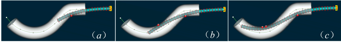
Figure 5.8: Computation of contact forces along the entire catheter robot for three configurations (a), (b) and (c).
