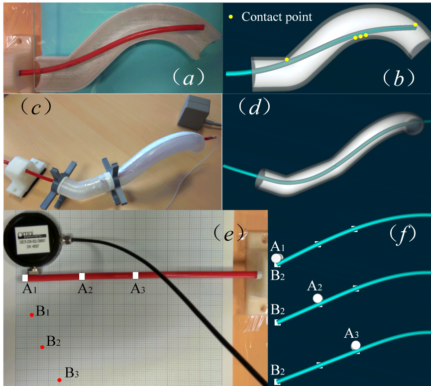
Figure 5.9: Experiment setup for the validation of the contact detection (( a ) and ( b )), the accuracy of simulation (( c ) and ( d )) and the contact force computation (( e ) and ( f )). In ( e ) and ( f ), A_1 - A_3 and B_1 - B_3 are respectively the contact locations and the desired positions of the tip.
