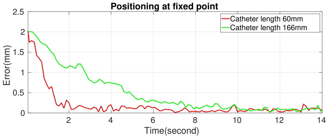
Figure 5.7: Convergence of positioning errors with different catheter length (60mm and 166mm).
