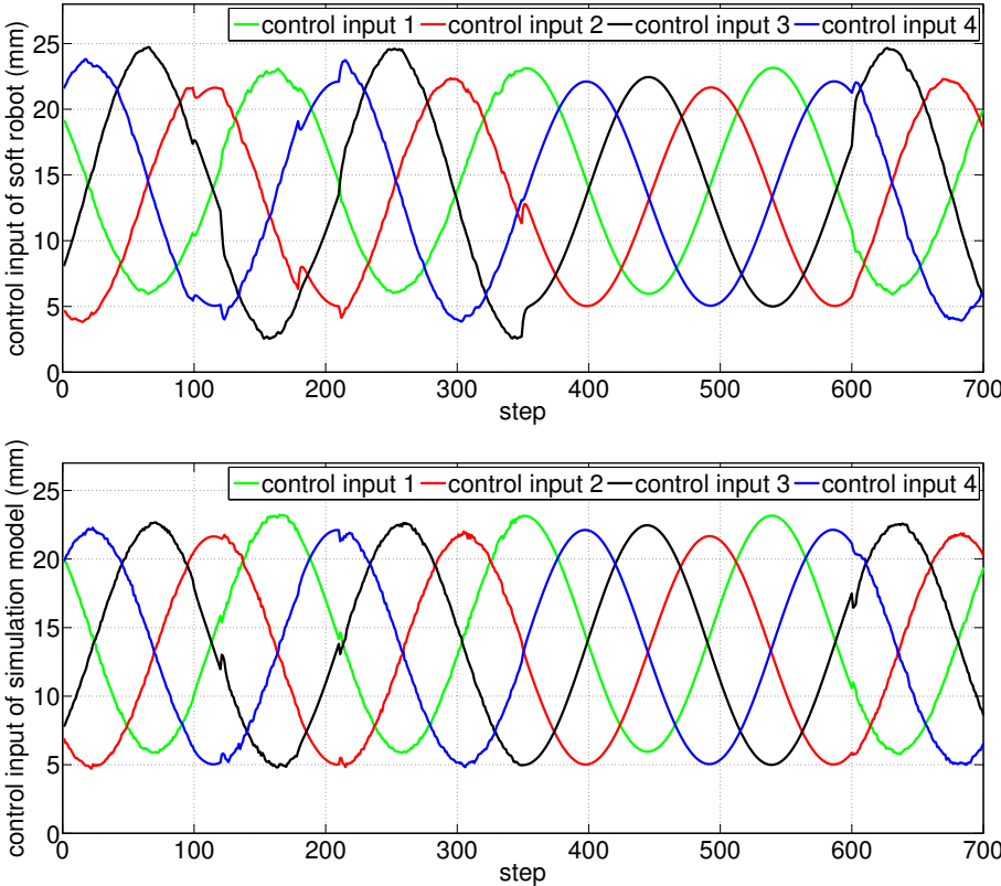
Figure 3.14: Tracking control inputs of soft robot and simulation model using the switched control strategy.
