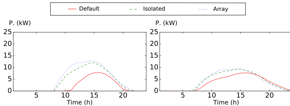
(a) Initial building Mean power needs: Default = 2.0 kW, Isolated = 3.9 kW, Array = 4.6 kW (b) Renovated building Mean power needs: Default = 3.2 kW, Isolated = 4.0 kW, Array = 3.9 kW
