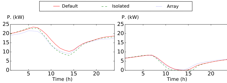
(a) Initial building Mean power needs: Default = 17.4 kW, Isolated = 16.5 kW, Array = 16.2 kW (b) Renovated building Mean power needs: Default = 4.7 kW, Isolated = 4.2 kW, Array = 4.5 kW
