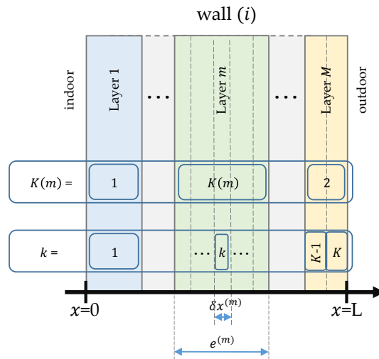
FIGURE 2.11: Wall notations
