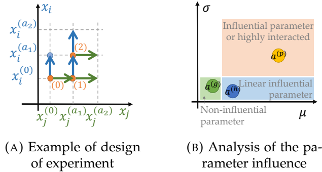
FIGURE 3.26: Morris method
