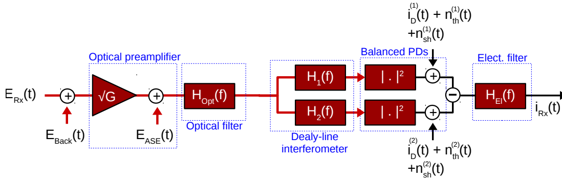
Figure 4.7: Baseband equivalent model of the DBPSK system.
