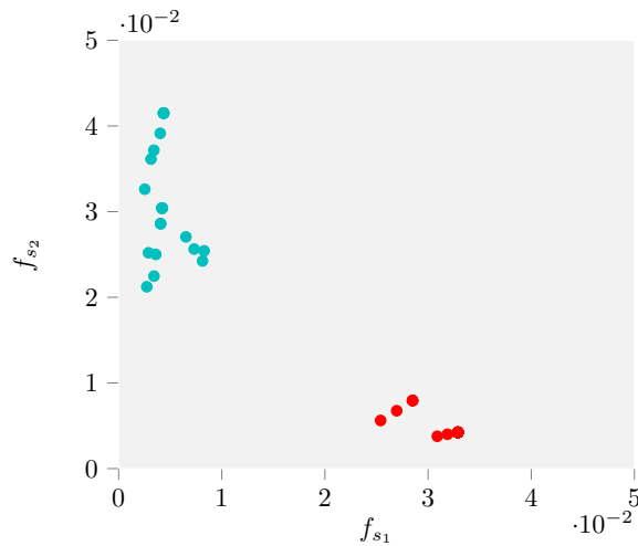
(c) Graph embedding using PPR
