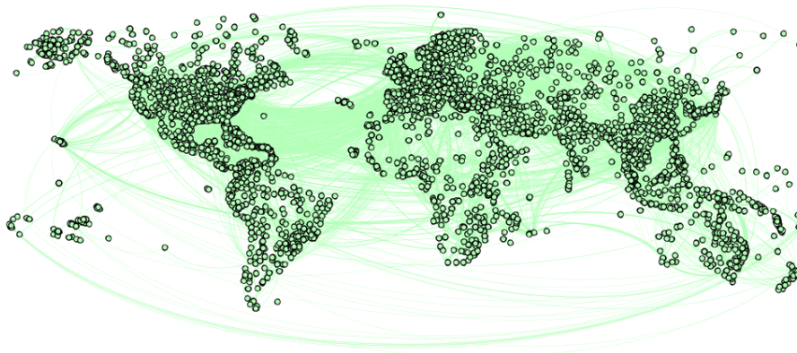
Figure 1.3: OpenFlights graph
