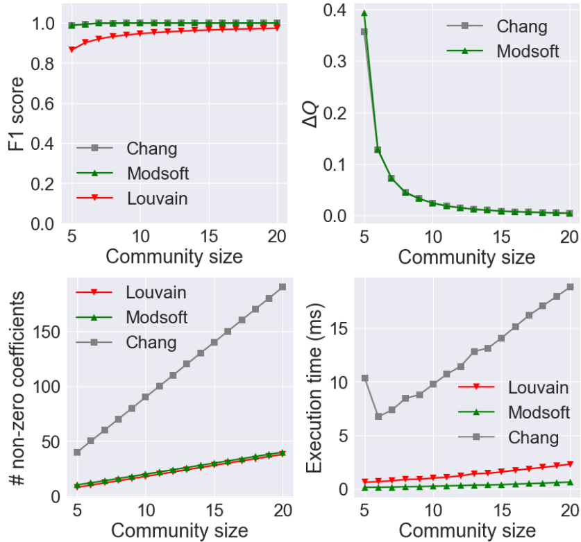
Figure 2.2: Overlapping SBM
