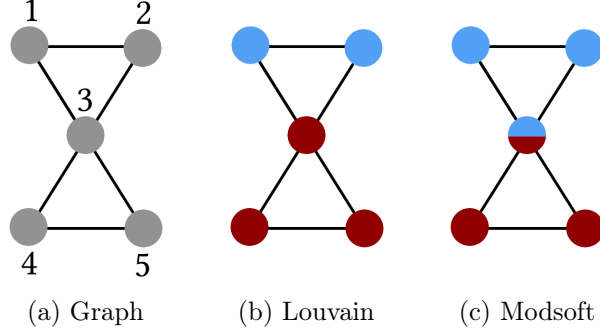
Figure 2.1: Bow tie graph
