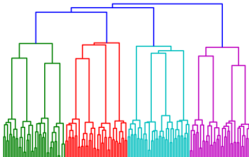
Figure 4.2: Dendrogram associated with the clustering of Paris on a hierarchical stochastic block model of 16 blocks.
