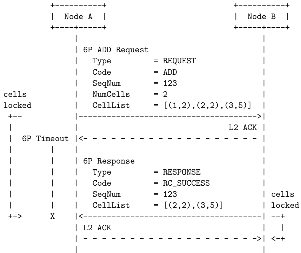
Figure 2.7: A 2-step 6P Transaction (borrowed from [25]).
