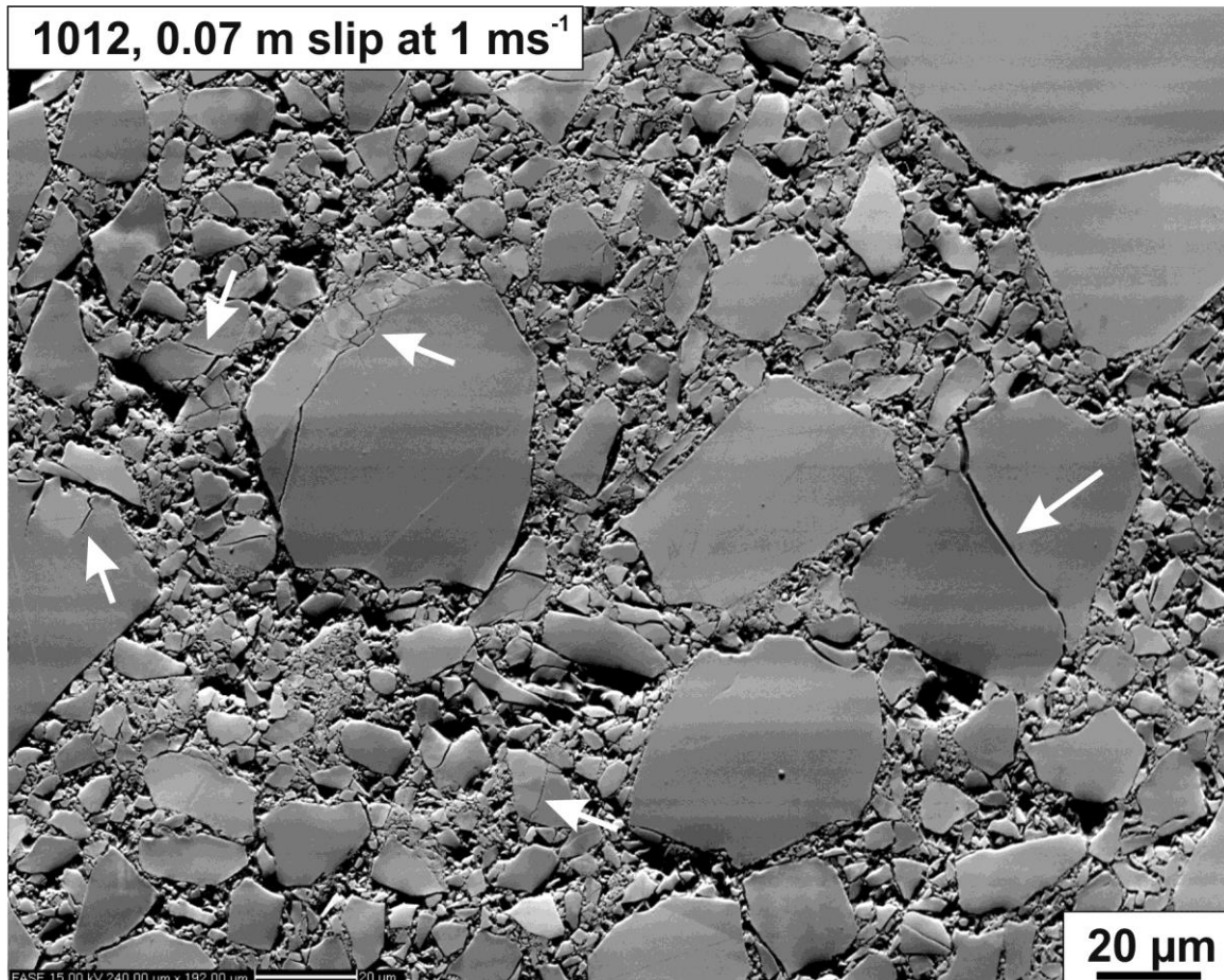
Fig. V-3 Forward scattered electron image from near the fine-grained zone in San Carlos olivine 1012.
