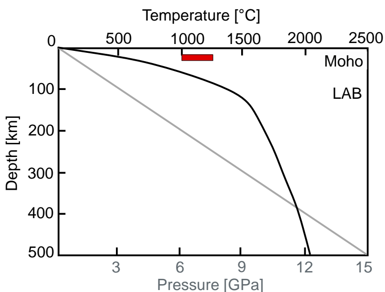
Fig. II-2 Temperature (black line) and pressure (grey line) curves for common crustal and mantle rocks. Areas shaded in grey show the position of the Mohorovičić discontinuity and Lithosphere-Asthenosphere boundary. The red rectangle shows conditions in the Paterson Press for deformation of olivine at strain rates of 10^{-5}\text{s}^{-1} . Geotherm after Earle (2016).
