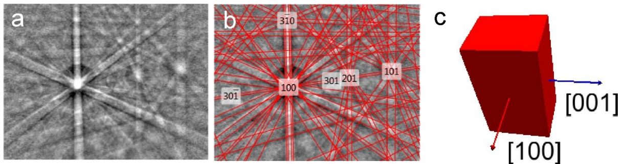
Fig II-9 (a) Exemplary Kikuchi pattern of forsterite (b) indexed bands representing certain crystal planes and the calculated crystal orientation (c) box model of the forsterite with lattice crystallographic orientation scaled to the unit cell dimensions.
