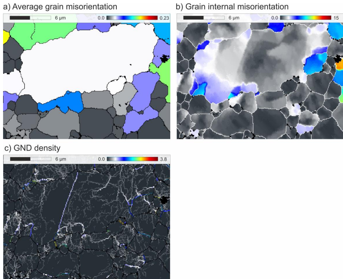
Fig. IV-3 Based on EBSD data, (a) average grain misorientation map, (b) internal misorientation relative to the grain gravity center and (c) density of geometrically necessary dislocations, for sample PI0546 deformed in torsion at 1200 °C and for 1.8 % of equivalent strain.
