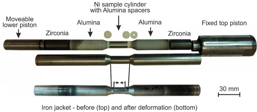
Fig. II-4 Image of a typical sample assembly. The bottom assembly experienced a deformation at 1200 °C to 8 % of strain. Note the lighter colors of the post-deformation Fe jacket towards the center and bottom, corresponding to the centered hot-zone.
