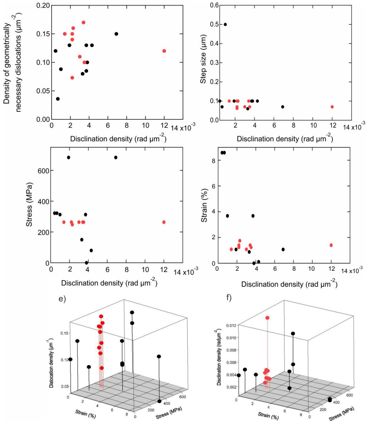
Fig. IV-6 Average disclination density as a function of (a) the density of GNDs, (b) EBSD map step size, (c) maximal stress and (d) finite strain and (e & f) 3-D scatter plots of the dislocation and disclination density as a function of stress and strain.
