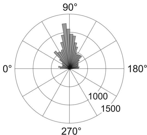
Fig. V-6 Rose diagram of the orientation of the long axis of the olivine grains to the shear axis. The sample of San Carlos olivine (1007) was deformed at 1 \text{ms}^{-1} to 1 m of slip and is representative for all deformed samples.
