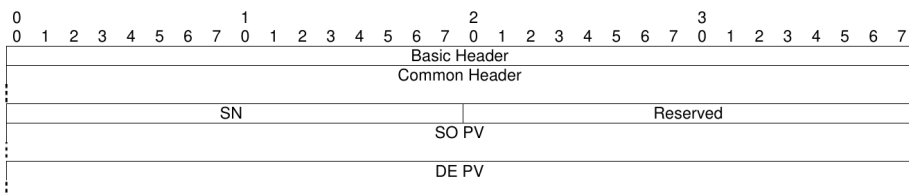
Figure A.4 – GeoUnicast structure
