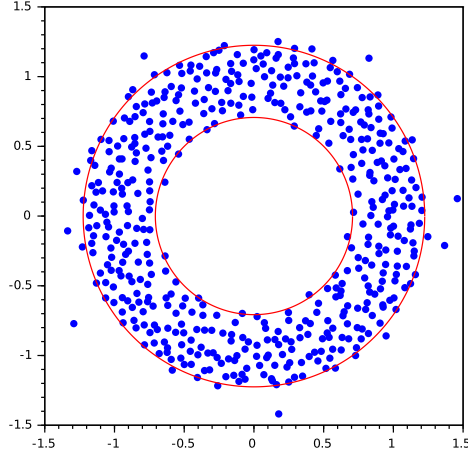
Figure 5.5: Eigenvalues of M_N where A_N = \text{diag}\left(e^{\frac{2i\pi}{N}}, \dots, e^{\frac{2iN\pi}{N}}\right) + \sqrt{N}f_N f_1^\top , with f_l = (e^{\frac{2i\pi lk}{N}}/\sqrt{N})_{1 \leq k \leq N} , N = 500 , \sigma^2 = 1/2 and X_N has complex Gaussian entries. For |z| > 1 , we have f_N^T R'_N(z) f_1 = 1/(z^N - 1) = o(1/\sqrt{N}) . The outlier eigenvalues in the unbounded component of the complement of \text{supp}(\beta) = \{z \in \mathbb{C} : 1/\sqrt{2} \leq |z| \leq \sqrt{3/2}\} converge in distribution to the zeros of 1 + \sigma g where g is the Gaussian analytic function with kernel H(z, w) = \varphi(z, w)^2/(1 + \sigma^2 \varphi(z, w)) and \varphi given by \varphi(z, w) = \frac{1}{1 - z\bar{w}} .
