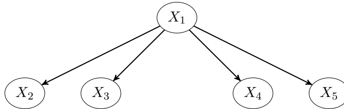
Figure 2.3: Representation of the tree G_{shallow}
