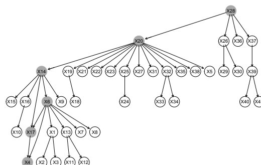
(f) BN learned with ds-BNSL on D_3
