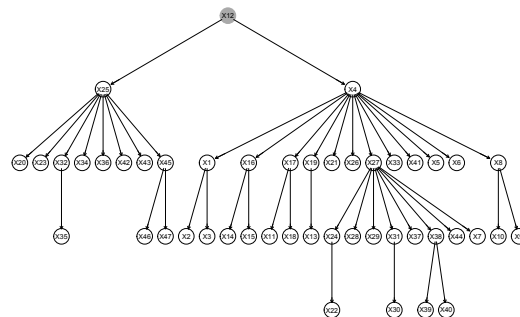
(b) BN learned with ds-BNSL on D_1
