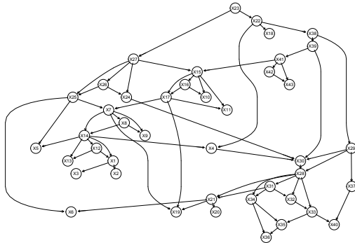
(c) BN learned with sota-BNSL on D_2
