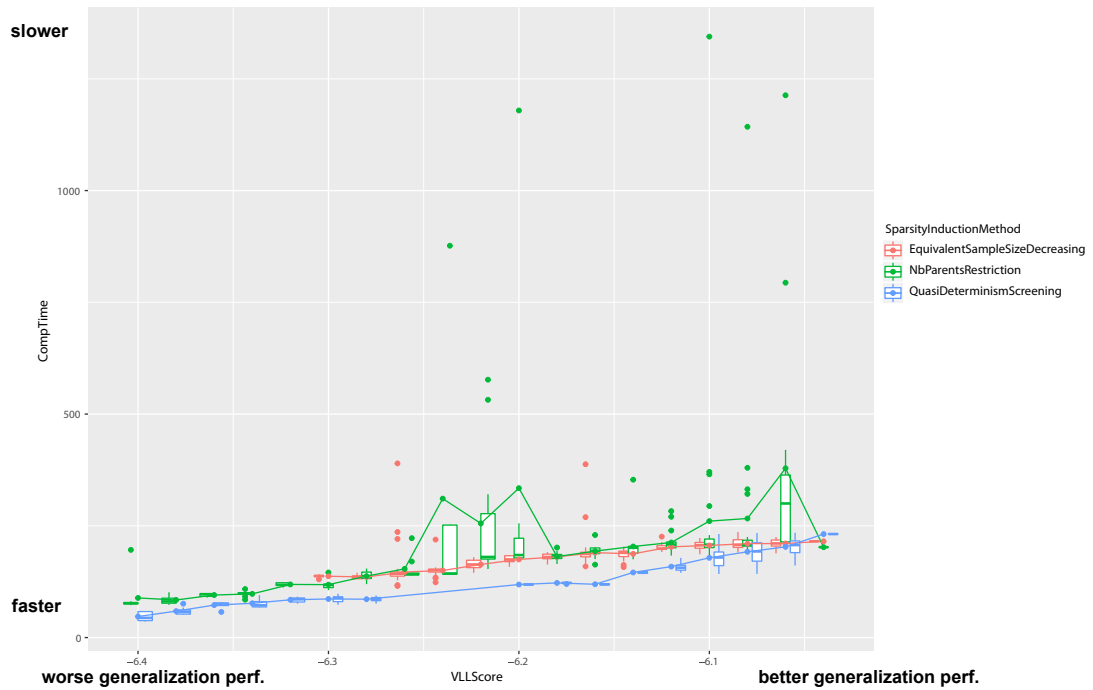
(b) performance/computation time tradeoff - msnbc dataset
