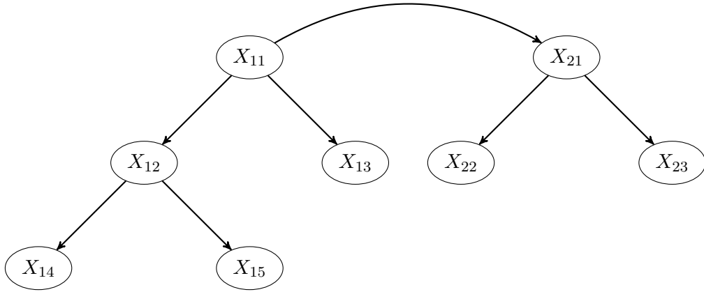
Figure 4.11: Graph G^*
