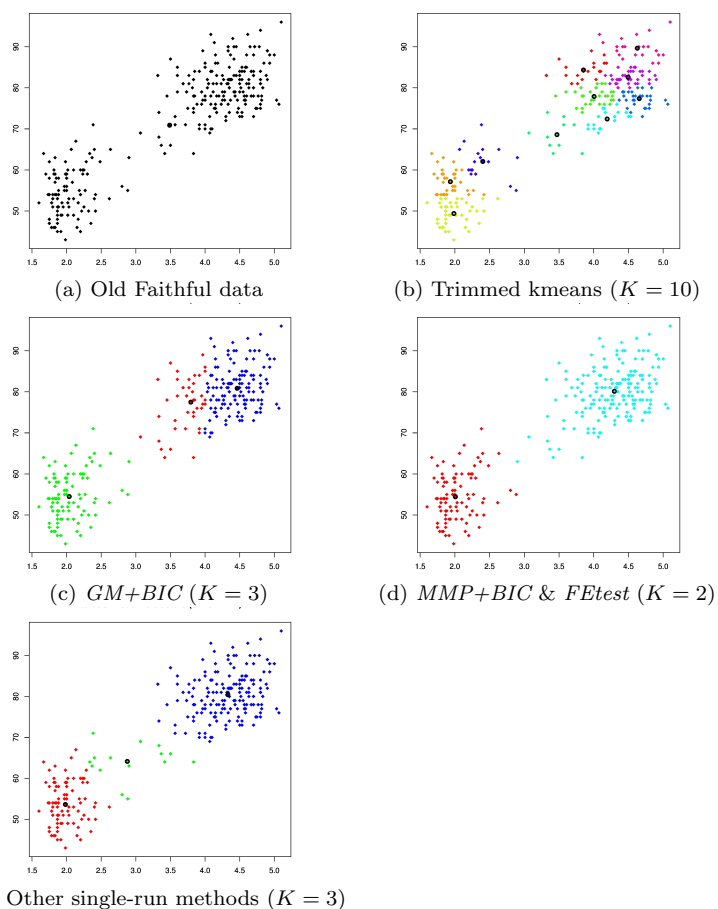
Fig. 3 (a): Old Faithful data, (b): 10 component initialization using trimmed k-means, (c): Gaussian mixture clustering as selected by BIC ( K = 3 ), (d): \mathcal{MP} clustering obtained with BIC and free energy based elimination ( K = 2 ); (e): \mathcal{MP} clustering for the other single-run procedures ( K = 3 ).
