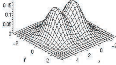
Figure 3.4: A Gaussian mixture model distribution in dimension d = 2 , with 2 gaussian components centered in [0, 0] and [3, 0] .
