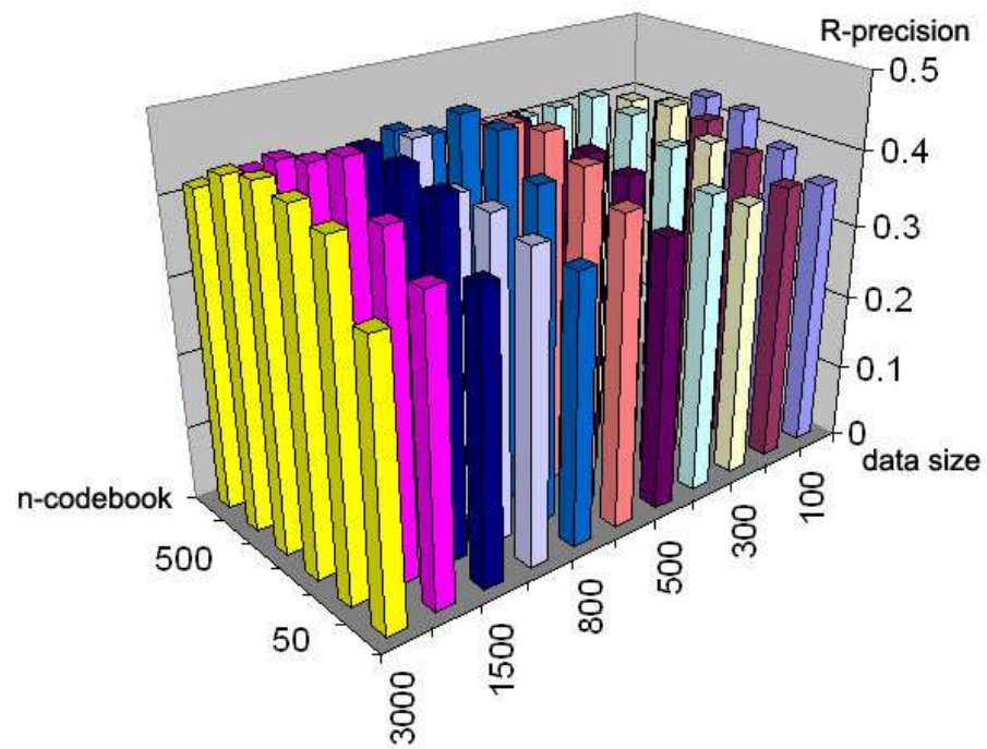
Figure B.7: Precision of Histogram comparison using Learning Vector Quantization for varying number of codebook vectors and training data size (per cluster) (using 100,000 iterations)
