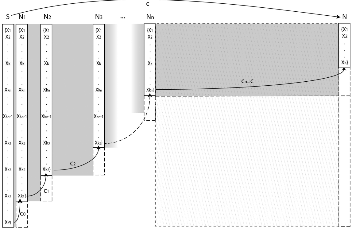
Figure D.2: Illustration of the algorithm. The cumulated cost of the successive steps appears as the light gray area, whereas the cost of the direct NN calculation appears as the stripped area.
