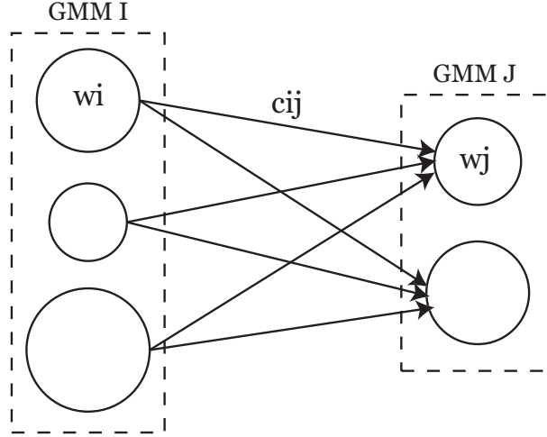
Figure B.4: Earth Mover's Distance between 2 Gaussian Mixture Models, viewed as a transportation problem between suppliers (components of GMM I ) and consumers (components of GMM J ).
