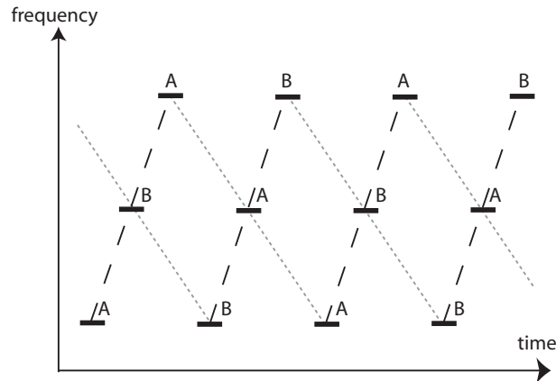
Figure 2.8: Classical Experiment illustrating the influence of timbre on stream segregation. A series of patterns of 3 ascending notes is presented to the subject. When the timbre distance between adjacent notes is small, the repeating ascending pitch line (dark-gray dashed) dominates the perception. If the distance between timbres of A notes and B notes increases, the notes are grouped by timbre similarity and 2 interleaved descending pitch lines are heard (light-gray dotted) (Wessel, 1991).
