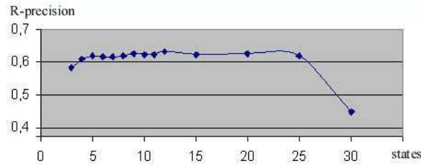
Figure B.6: Influence of the number of states in HMM modelling
