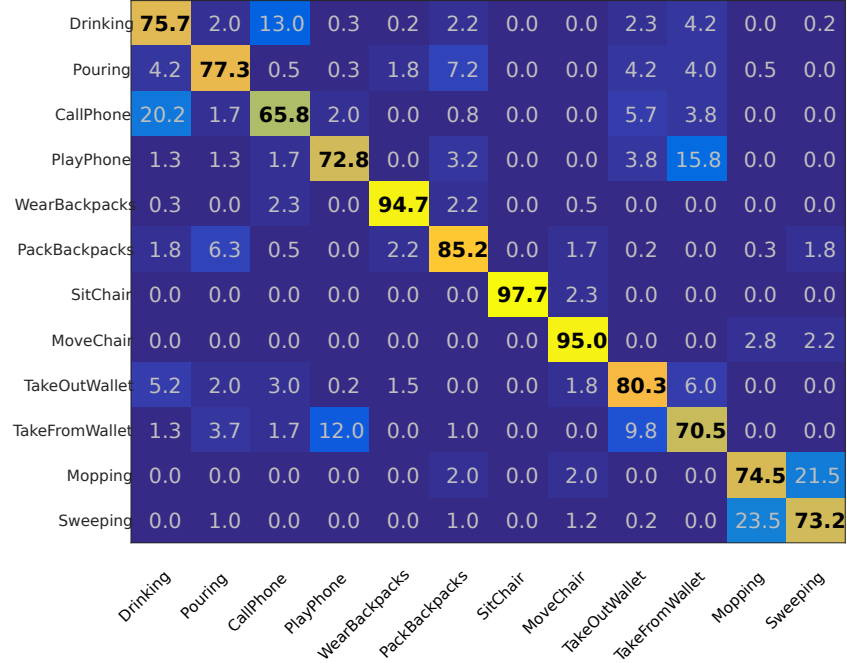
FIGURE 3.8 – Confusion matrix for the SYSU3D dataset.
