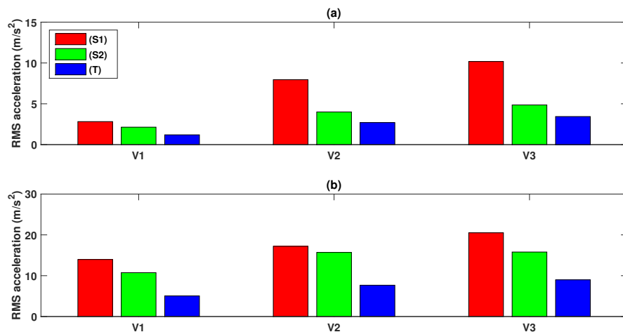
Fig. 6.6 RMS values of hand's 3D acceleration for different walking conditions: (a) experimental data, (b) simulation data.
