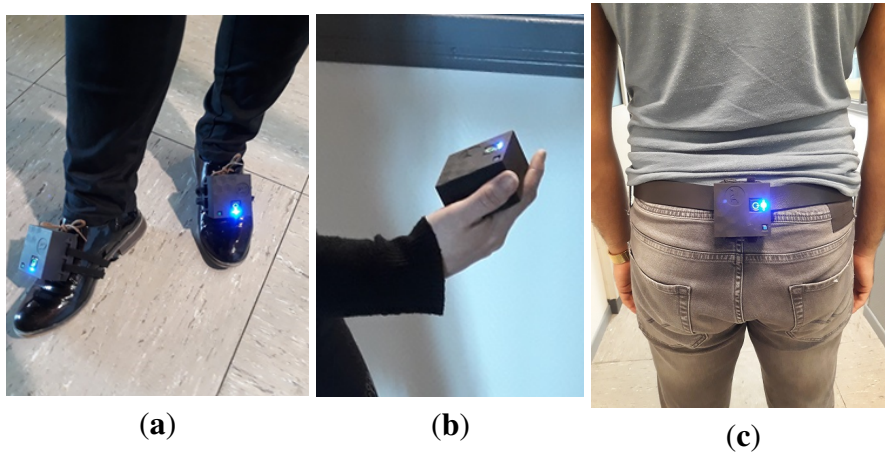
Fig. 3.1 Placement of different devices during walking trials: (a) PERSYs; (b) ULISS 1; (c) ULISS 2.
