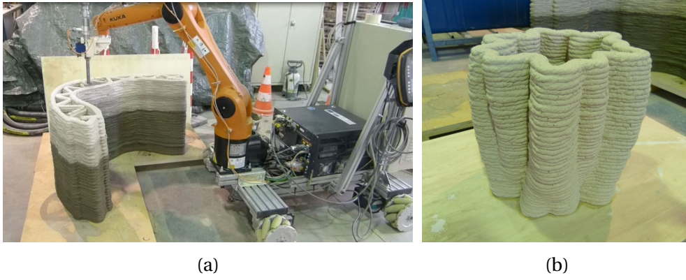
Figure A.12 – 3D printing on November 17, 2017 - ENSAPL
