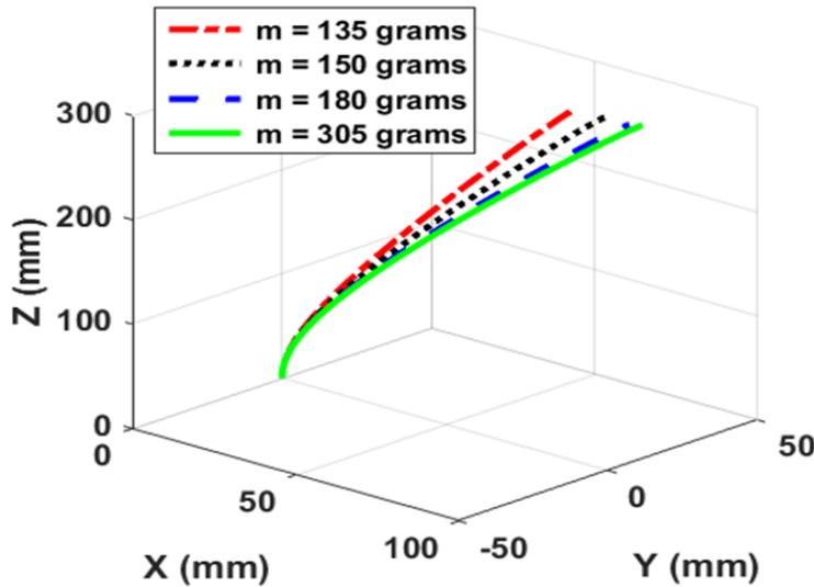
Figure 4.11: Effect of mass on the shape of CBHA manipulator
