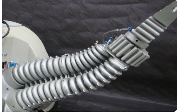
Figure 3.16: CBHA manipulator with two inflection points
