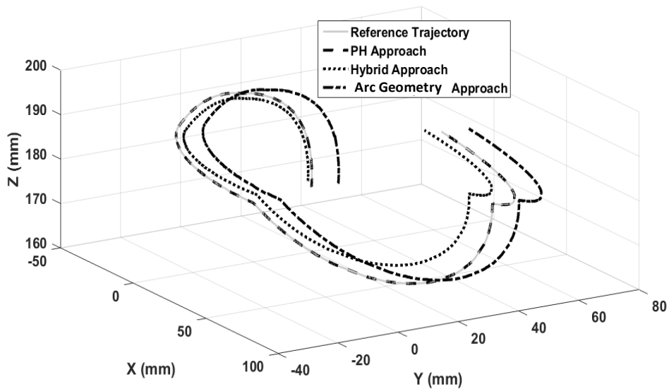
Figure 4.14: Trajectory tracked using FKM
