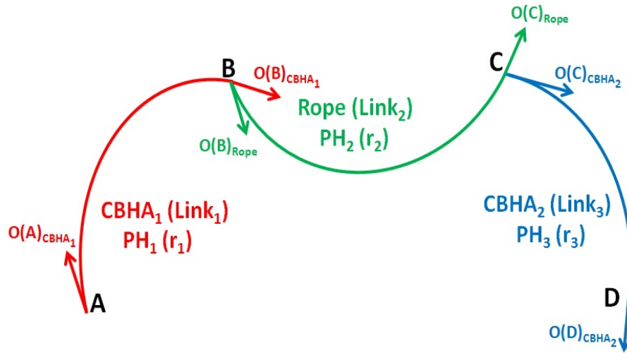
Figure 5.5: Modeling of closed loop kinematic chain using PH curves
