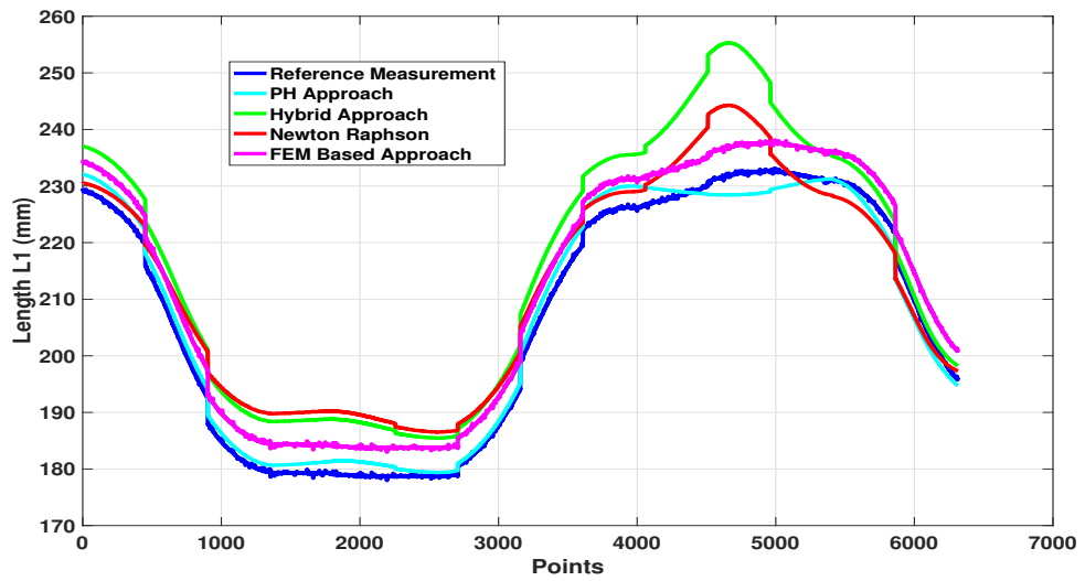
Figure 4.7: Comparison of length L1
