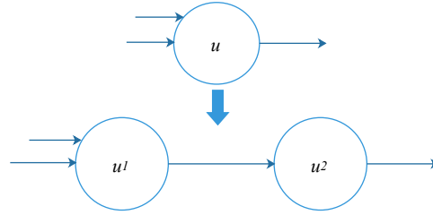
FIGURE 6.5: Node splitting [244]
