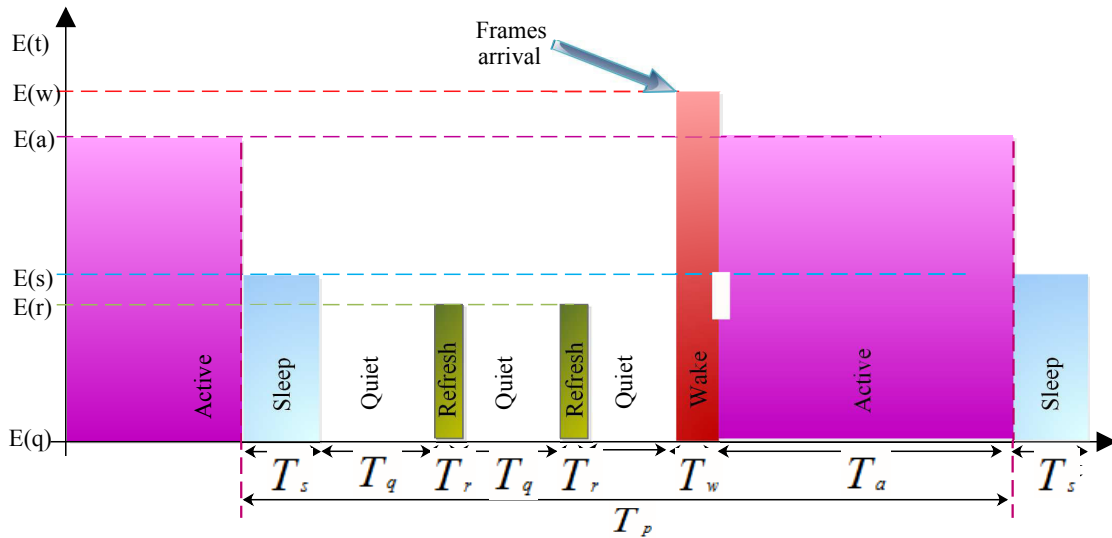
FIGURE 2.2: Relative power consumption for different periods of EEE
