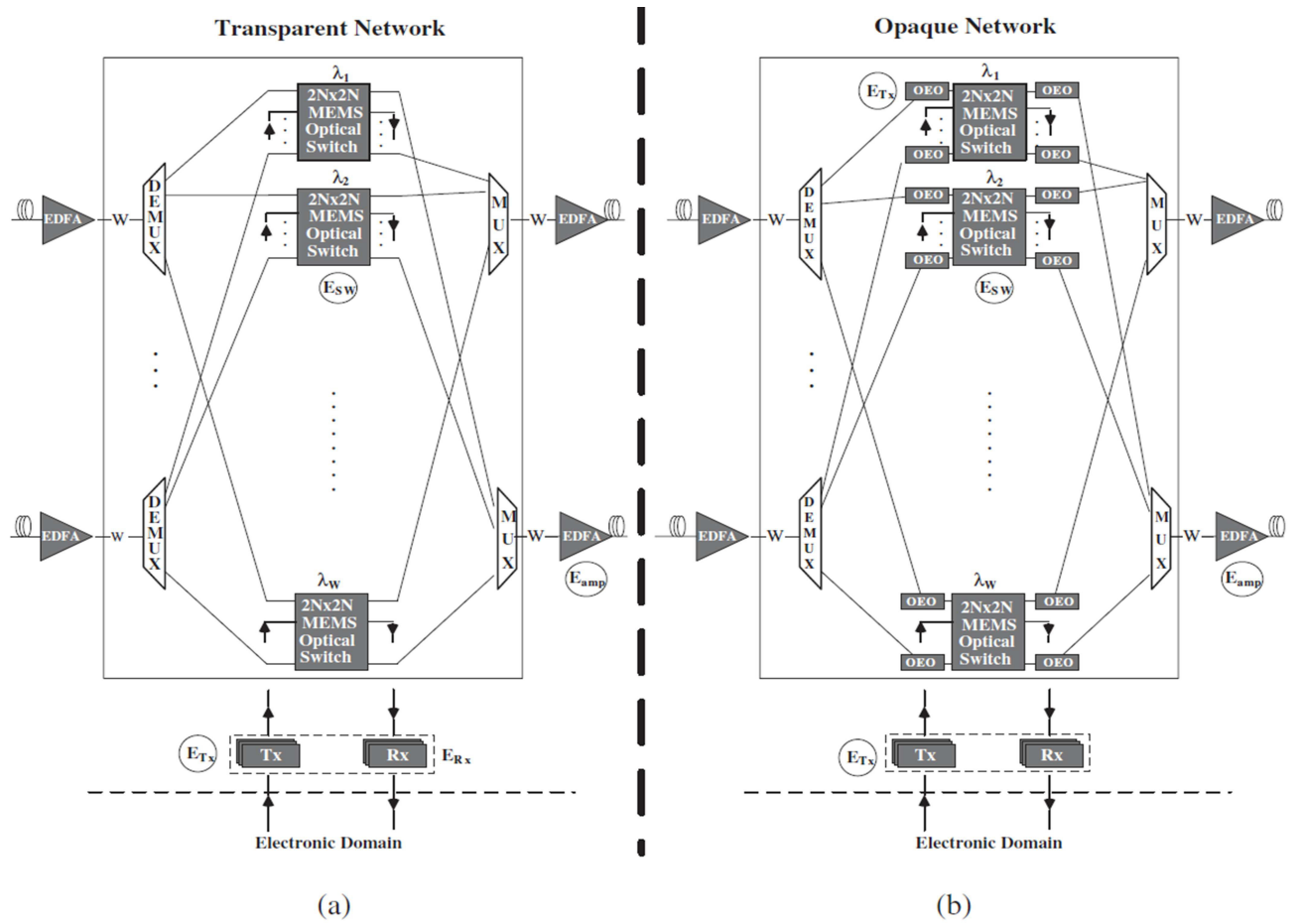
FIGURE 1.10: OXC architecture [79]
