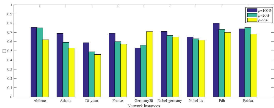
FIGURE 5.16: Fairness index versus \rho using TM1 with the MP-MP heuristic
