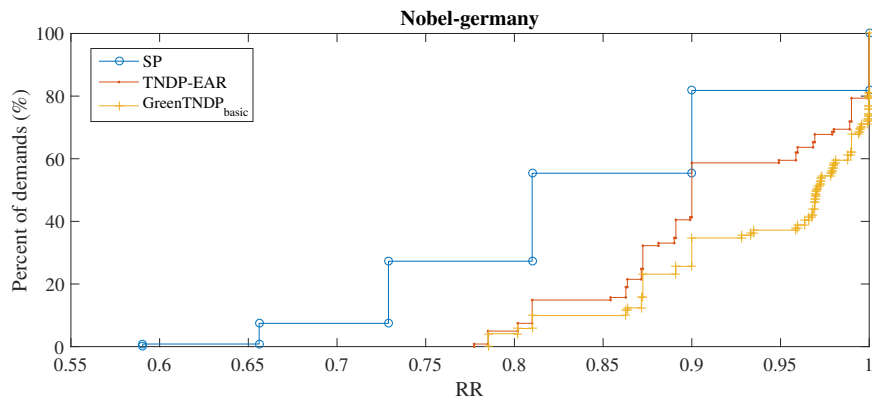
FIGURE 6.18: CDF of routing reliability on Nobel-germany
