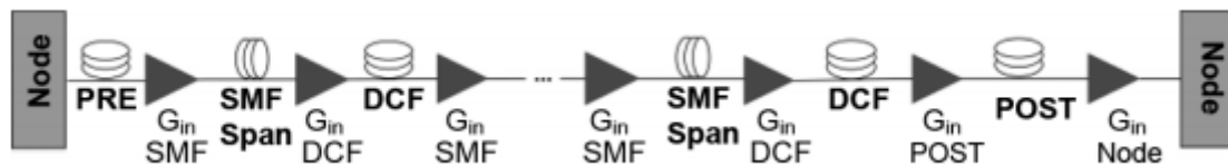
FIGURE 1.11: Fiber link model [79]
