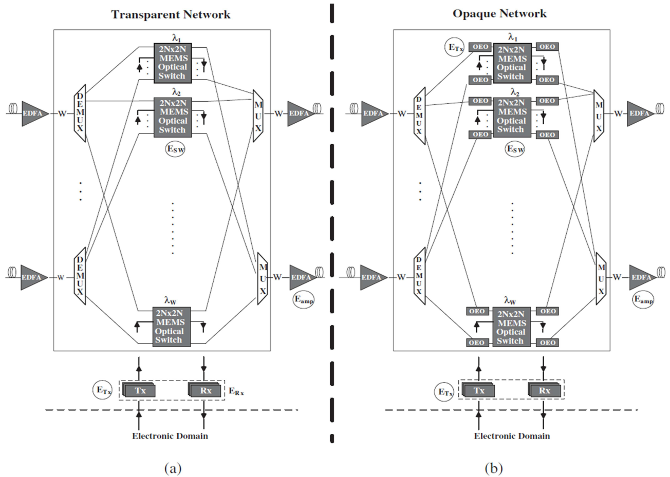
FIGURE 1.10: OXC architecture [79]
