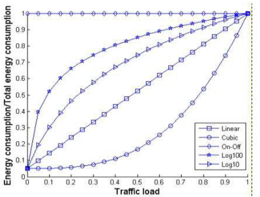
FIGURE 1.5: Proposed Energy Profile [56]
