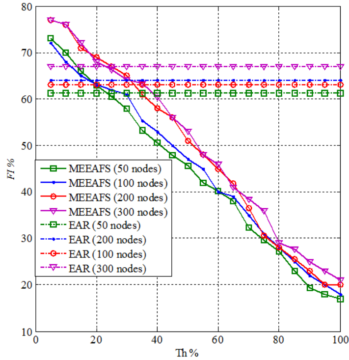
FIGURE 3.10: Fairness index versus link load threshold at medium load
