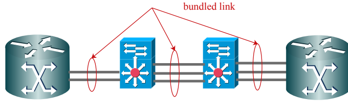
FIGURE 4.2: Bundled links
