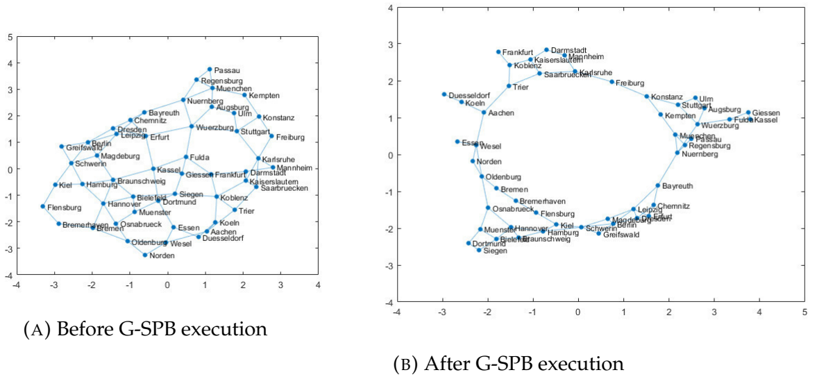
FIGURE 4.10: Germany50 network
