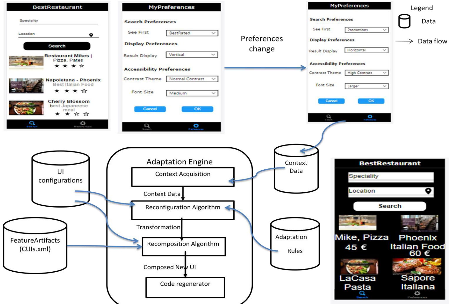
Figure 4-8 The Runtime Adaptation Mechanism
