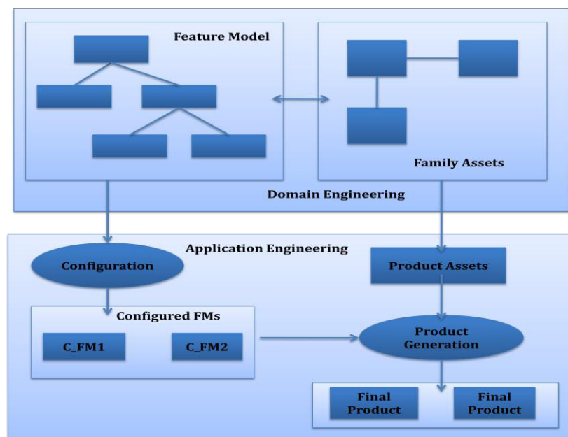
Figure 1-0-4. Software Product Line Process
