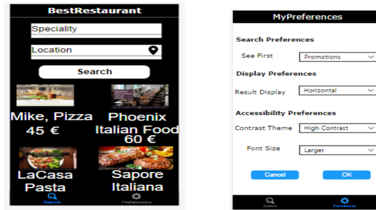
(a) The search UI after Adaptation (b) the new preferences Settings
