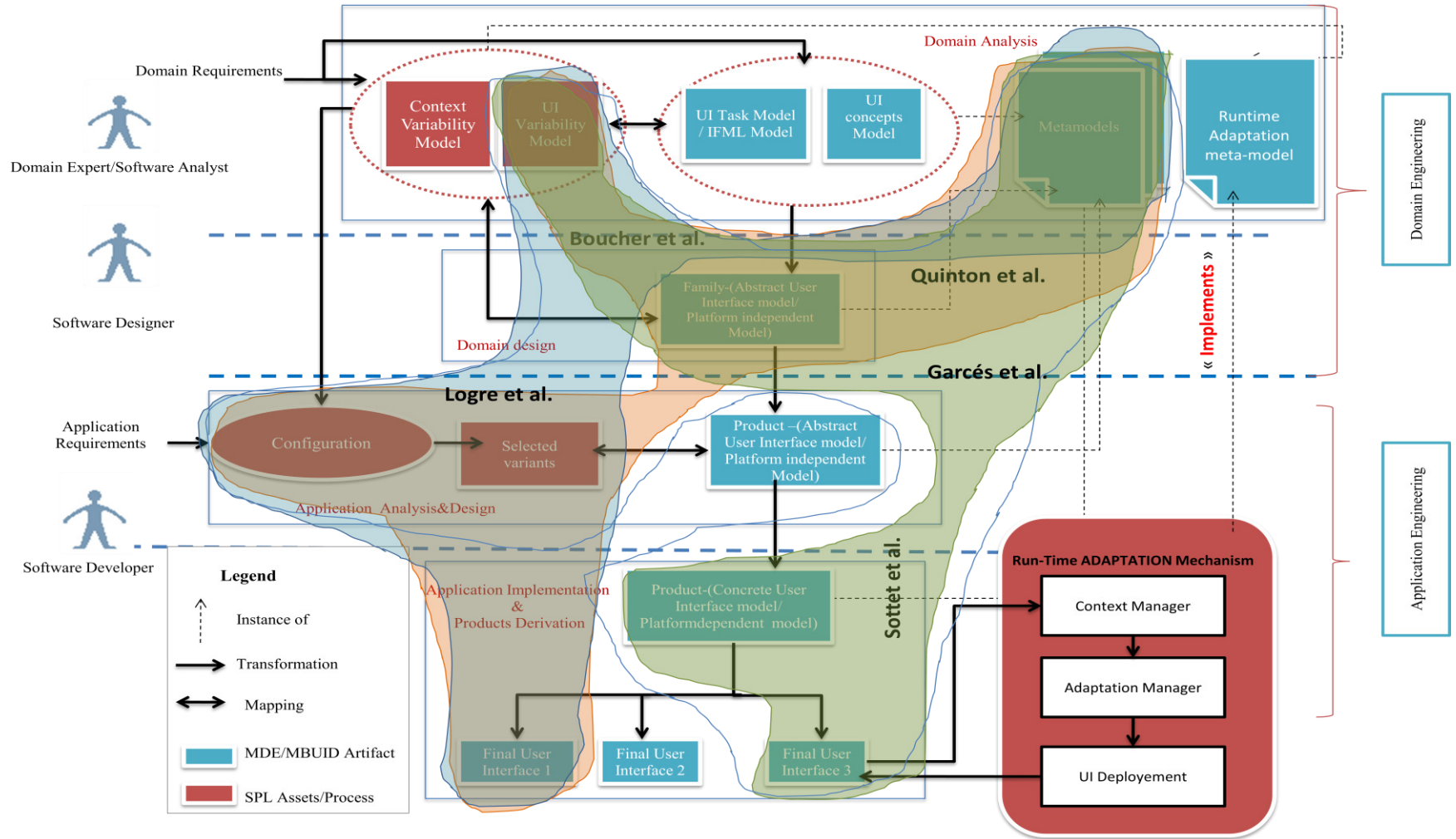
Figure 0-8 The tagging of existing works-Part 2
