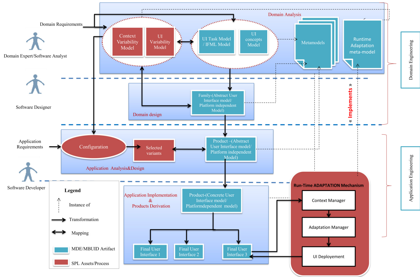
Figure 0-6 A summary/reference schema for the development of user interfaces using SPL and MDE core assets
