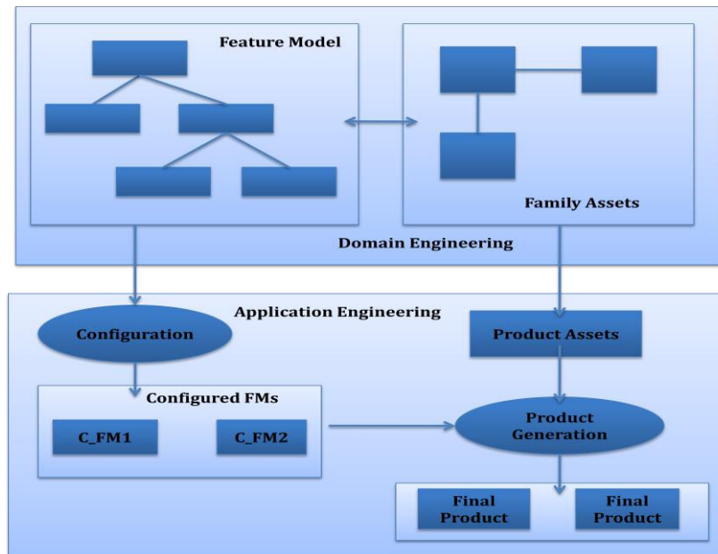
Figure 0-4. Software Product Line Process
