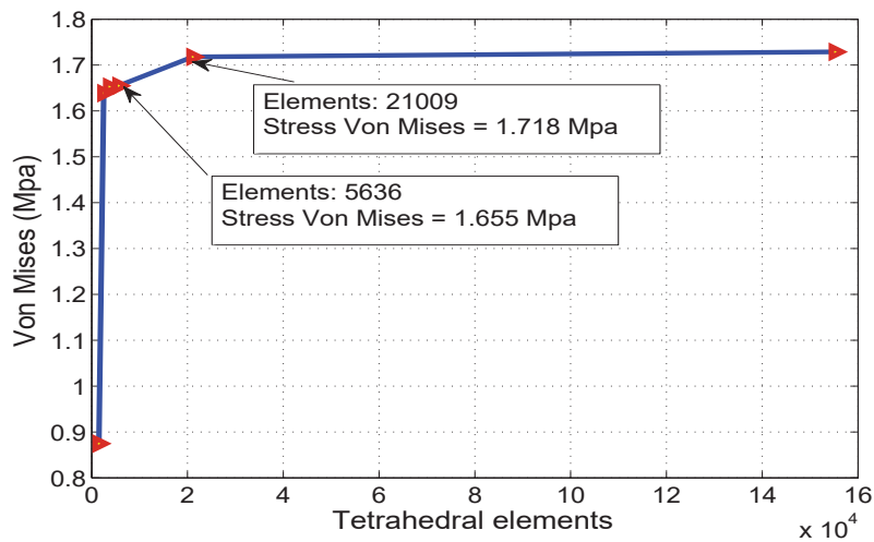
Figure 4.5 – Mesh convergence study: Stress Von Mises computed for different resolution of meshing.
