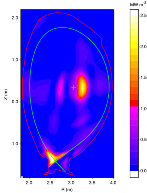
Figure 6.1.: Poloidal reconstruction of radiative power loss in a JET discharge [57]. This radiative power is attributed to impurity.
