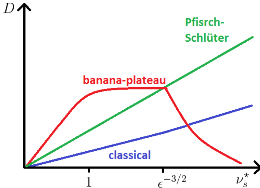
Figure 4.3.: Comparison between the classical prediction (blue), the banana-plateau contribution (red) and the Pfirsch-Schlüter contribution (green)
