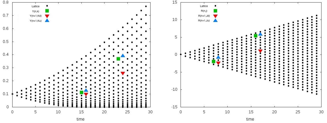
Figure 3.1: The tree for the process Y (left) and for R (right), showing as the trees may be visited.
