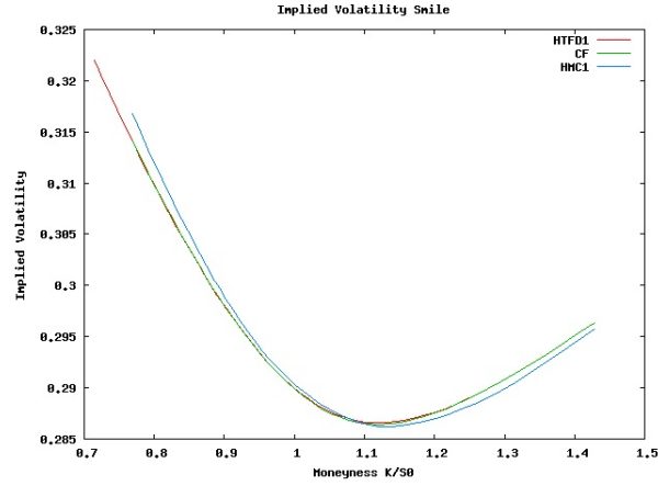
Figure 3.2: Standard Bates model. Moneyiness vs implied volatility for European call options. Test parameters: T = 0.5 , r = 0.03 , \delta = 0.05 , Y_0 = 0.04 , \theta_Y = 0.04 , \kappa_Y = 2 , \sigma_Y = 0.4 , \lambda = 5 , \gamma = 0 , \eta = 0.1 , \rho = -0.5 .
