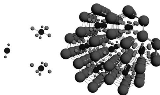
Fig. 2 Steps in the WFT-in-DFT embedding calculation on the f - f spectrum of \text{Cs}_2\text{U}(\text{Np})\text{O}_2\text{Cl}_4 . From left to right, (a) the initial \text{NpO}_2^{2+} ion (b) is surrounded by four chlorides (top: chlorides considered explicitly in the WFT calculations; bottom: ligand group \text{Cl}_4^{4-} is taken as part of the environment and included via the embedding potential) to make up the central unit in the cluster model; and (c) this unit is embedded into a larger environment. The larger model is then embedded in an array of point charges (not shown).
