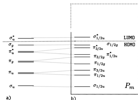
FIG. 1. Diagram of valence molecular orbitals of the triiodide ion, arising predominantly from the 5p manifold of the three iodine atoms: (a) spin-orbit free case and (b) spin-orbit case with the model P_m space employed in the IHFSCC calculations indicated.
