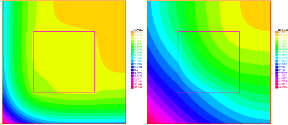
Figure 4.7 – Test case (b) : Synthetic true solutions with Neumann boundary conditions. Left: \mu = 1 in D_{\text{syn}}(\mu) (values from 17.4^{\circ}\text{C} to 117.9^{\circ}\text{C} ). Right: \mu = 20 in D_{\text{syn}}(\mu) (values from 29.8^{\circ}\text{C} to 44.3^{\circ}\text{C} ).
