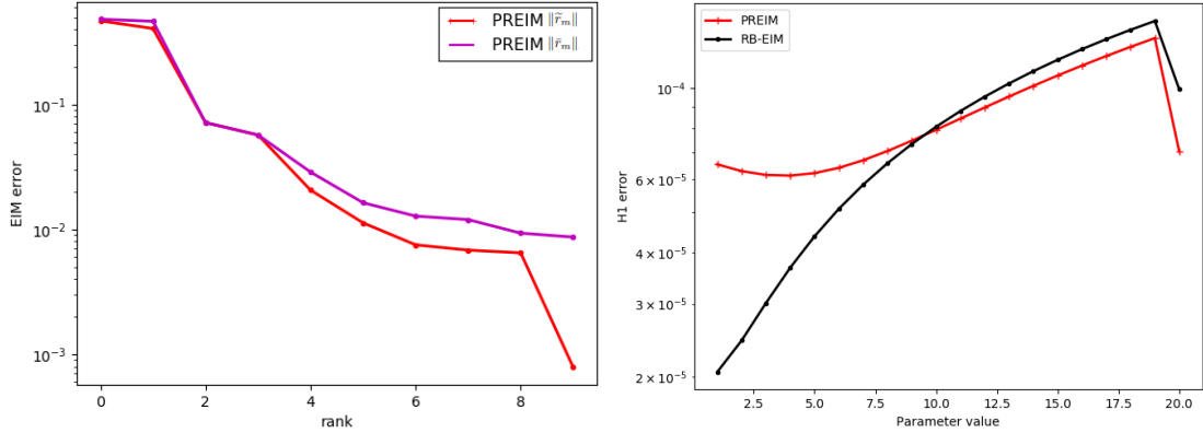
Figure 2.13 – Test case (c): Left: EIM approximation errors \|\tilde{r}_m\|_{\ell^\infty(\Omega^{\text{tr}})} and \|\bar{r}_m\|_{\ell^\infty(\Omega^{\text{tr}})} as a function of m for PREIM with \epsilon_{\text{POD}} = 10^{-4} and \epsilon_{\text{EIM}} = 5 \cdot 10^{-3} . Right: RB approximation error \|u_\mu - \hat{u}_\mu\|_{\ell^2(I^{\text{tr}}; H^1(\Omega^{\text{tr}}))} / \|u_\mu\|_{\ell^2(I^{\text{tr}}; H^1(\Omega^{\text{tr}}))} for \epsilon_{\text{POD}} = 10^{-3} and \epsilon_{\text{EIM}} = 5 \cdot 10^{-3} .
