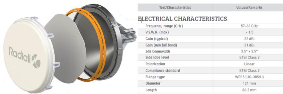
Figure 2-54: Commercialized V-band transmit-array (Radiall) [109].
