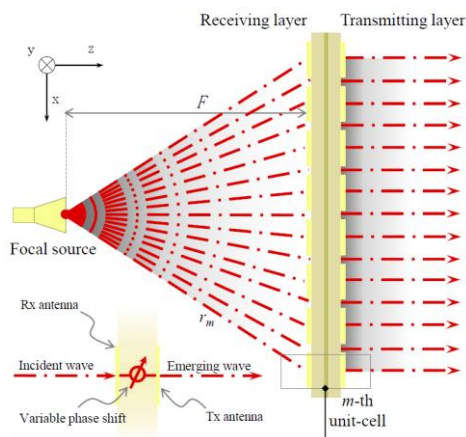
Figure 2-42: Principle of Transmit-array [86].
