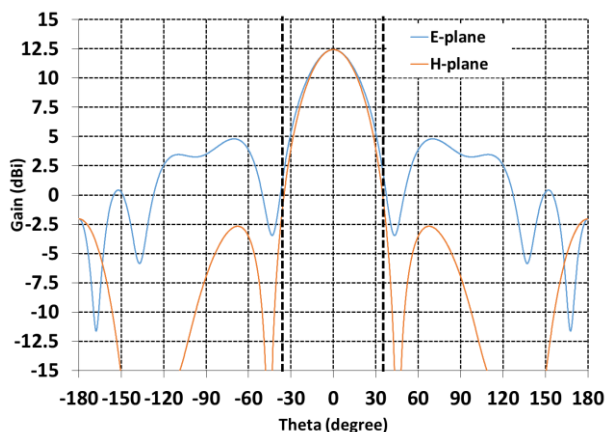
Figure 4-21: Radiation patterns of a 2x2 sub-array of ACMP elements with separate feeding line per element.
