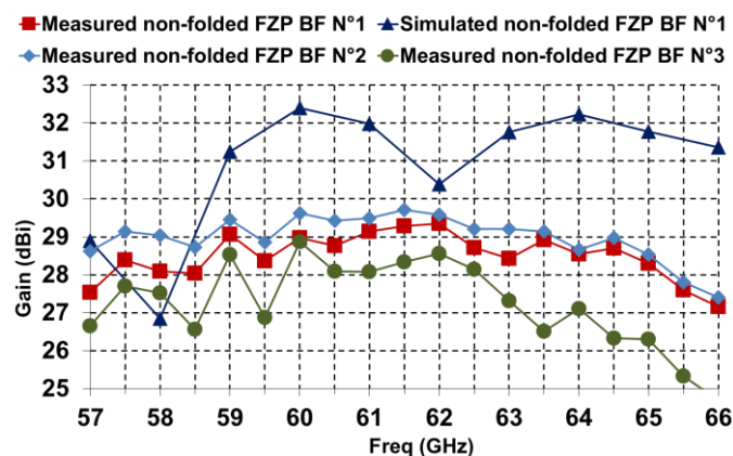
Figure 5-29: Measured and simulated gain variation over frequency for non-folded FZP fed by continuous beam steering tapered focal arrays.
