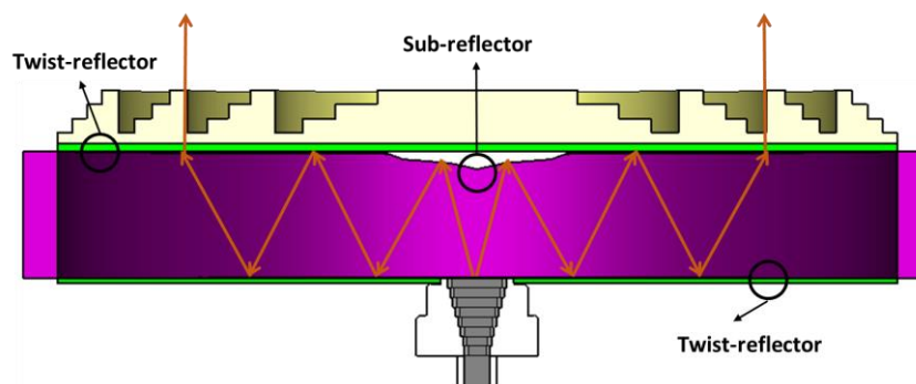
Figure 6-13: Cross-section of the Triple Folded FZP lens antenna structure.
