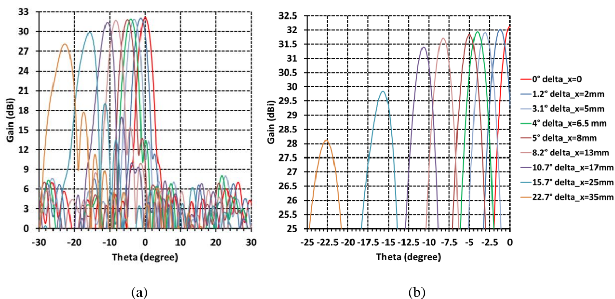
Figure 4-4: FFZP antenna beam steering for different primary source (waveguide aperture) positions on x -axis of the focal plane at 60 GHz : (a) Wide angle view diagrams, (b) Zoomed view diagrams.
