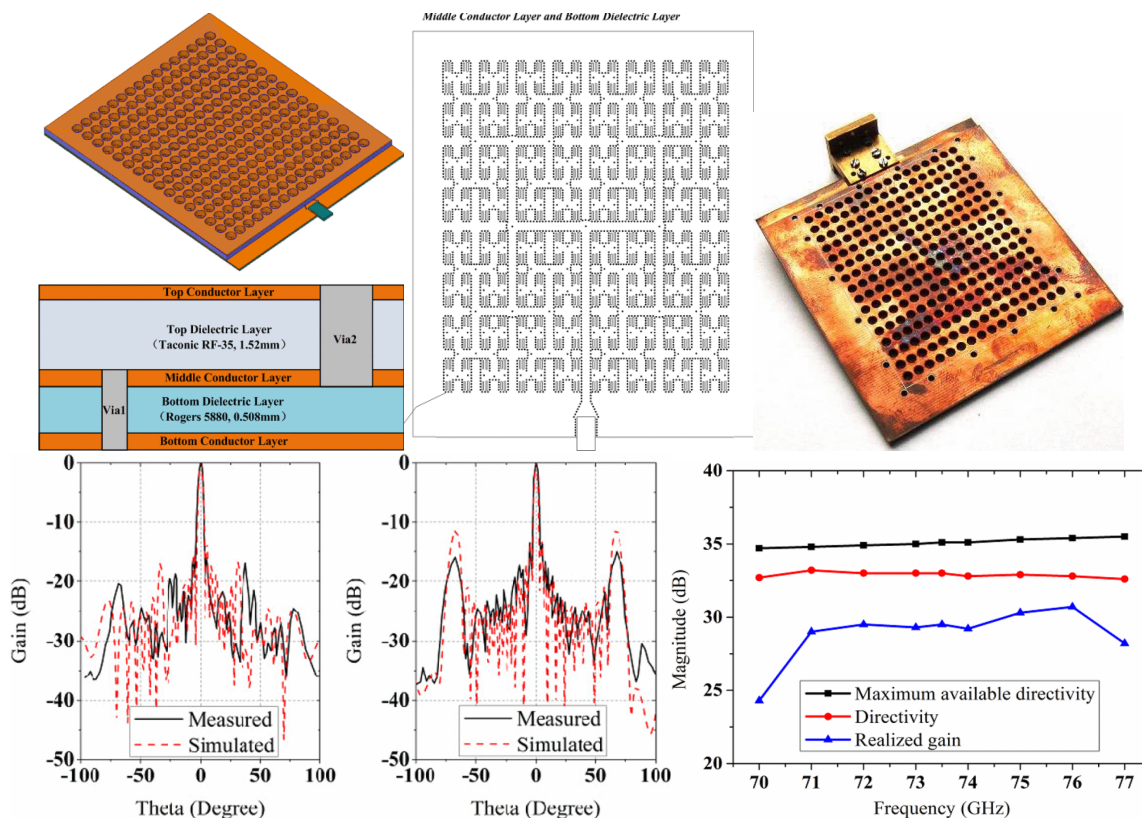
Figure 2-22: 16x16 SIW antenna array for E-band [27].
