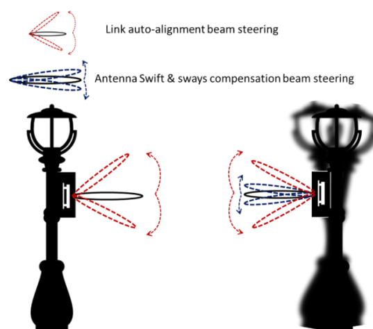
Figure 4-1: Backhaul antenna beam steering scenarios.
