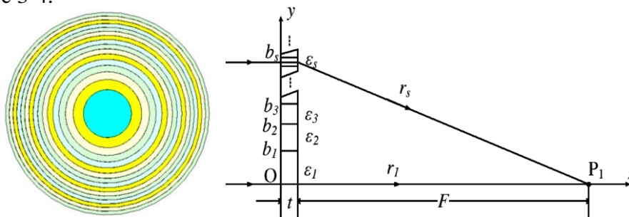
Figure 3-4: Multi-dielectric FZP lens.
