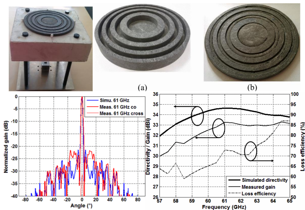
Figure 2-36: V-band Fresnel Zone plate lens antenna with foam technological process [70].
