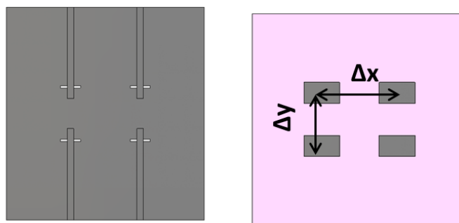
Figure 4-20: ACMP 2x2 sub-array structure.
