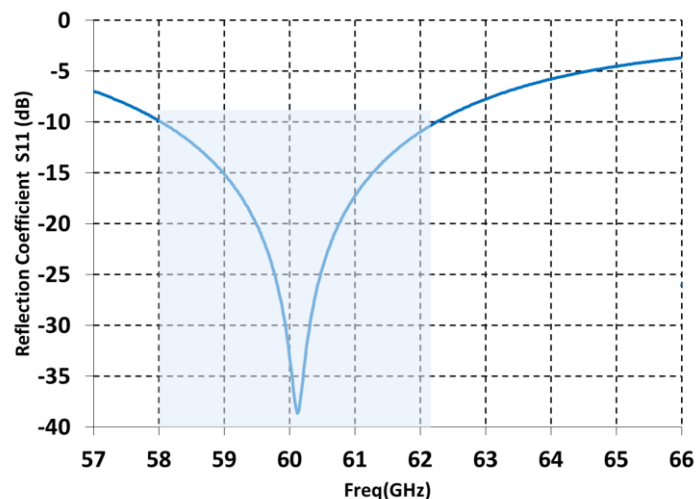
Figure 4-9: Reflection coefficient of the simple Aperture Coupled Microstrip Patch antenna.
