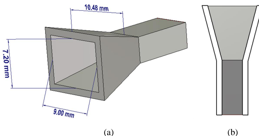
Figure 3-15: Optimal edge taper horn N3 : (a) 3D perspective view, and (b) and cut-view.
