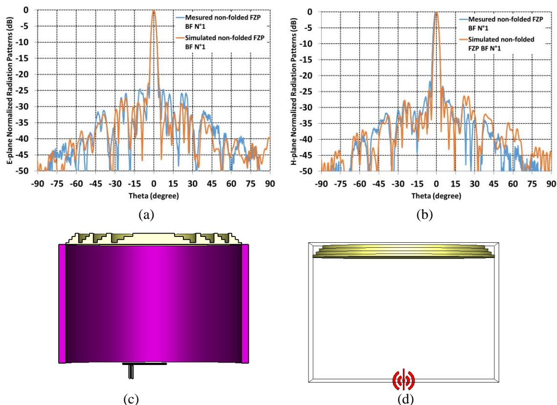
Figure 5-27: Measured and simulated radiation patterns of the non-folded FZP fed by uniform amplitude 2 \times 2 focal array ( N^{\circ}1 ) (a) E-plane, (b) H-plane, (c) CST time domain solver simulation model of the non-folded FZP and circuit N^{\circ}1 and N^{\circ}2 , and (d) CST IE solver simulation model of the non-folded FZP lens and imported far fields of circuits N^{\circ}3 .
