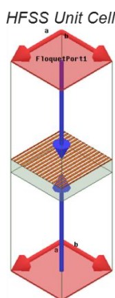
Figure 3-22: Trans-reflector unit-cell.
