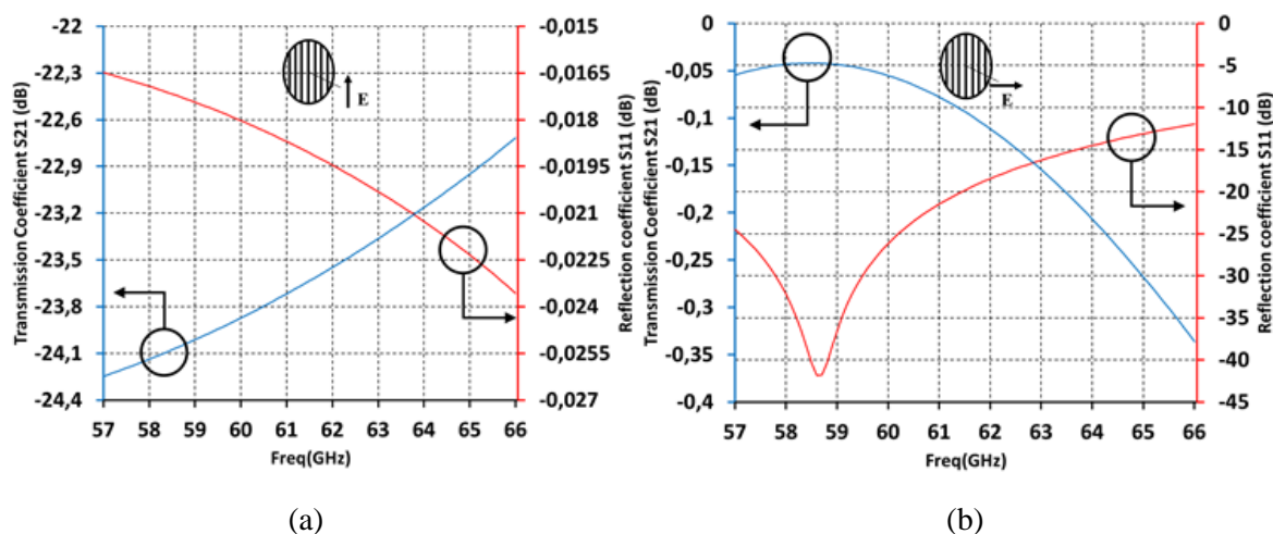
Figure 3-23: Trans-reflector reflection and transmission simulated coefficients : (a) Parallel linear polarized incident wave, (b) Perpendicular linear polarized incident wave.
