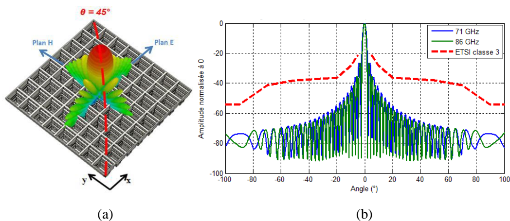
Figure 2-8: 32×32 stepped horn elements array : (a) 3D schematic and radiation pattern, and (b) normalized 45° plane radiation patterns at 71 GHz and 86 GHz superimposed by ETSI class 3 RPE [6].
