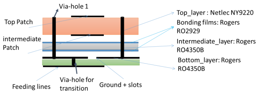
Figure 5-4: Primary design of ACMP with isolating via-holes layout.
