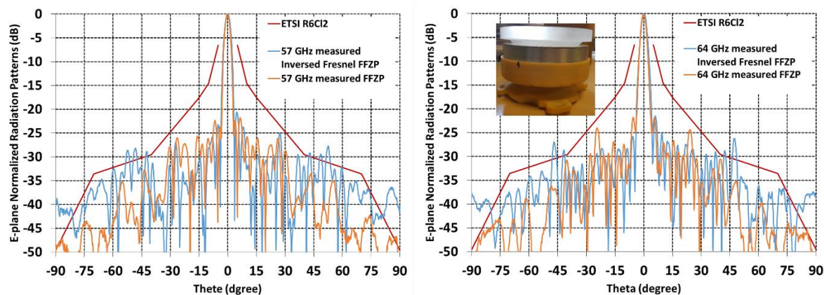
Figure 3-34: E-plane normalized measured radiation patterns of the FFZP antenna for Inversed and non-inversed FZP lenses.
