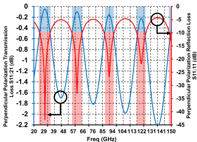
Figure 6-7: Trans-reflector harmonics of reflection loss and transmission loss for perpendicular polarized incident waves.
