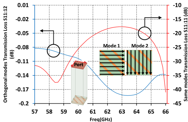
Figure 3-36: Optimized Twist-reflector modal transmission coefficients. The HFSS unit-cell, the Floquet port, and the two orthogonal modes are shown in the inset.
