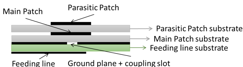
Figure 4-11: Aperture Coupled Microstrip Patch Antenna with parasitic patch (ACMPP) side-view schematic.
