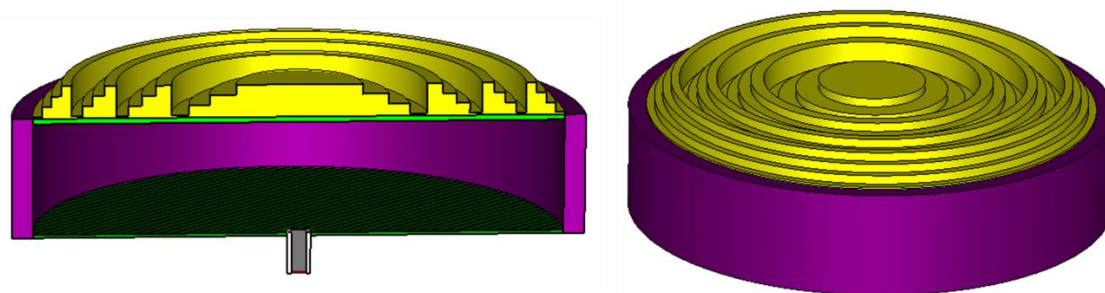
Figure 3-37: FFZP antenna simulation 3D structure with the lens (made of PP or PMMA).
