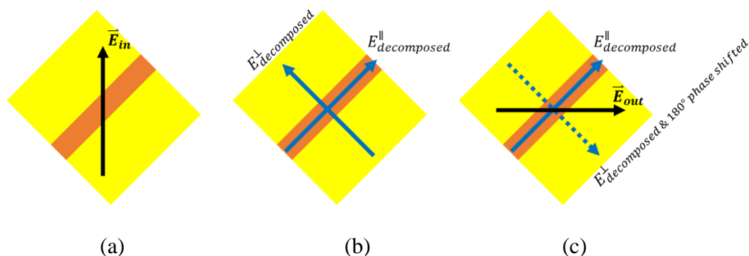
Figure 3-25: Twist-reflector functionality based on vector field decomposition: (a) Incident wave, (b) decomposition of incident wave into parallel and perpendicular components, and (c) Composition of the parallel component reflected directly and perpendicular component reflected with 180° phase shift resulting in the reflected wave with 90° polarization twist.
