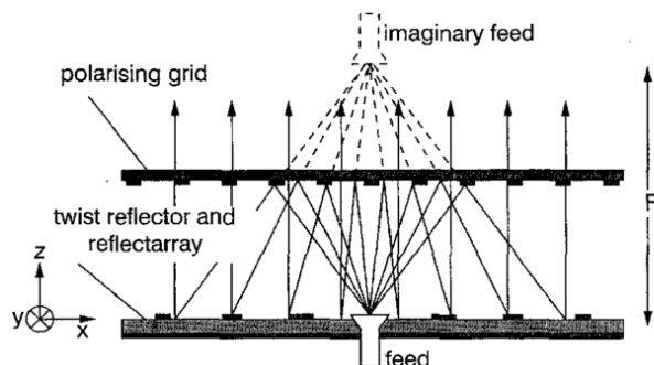
Figure 2-40: Principle of the folded Reflect-array antenna [84].
