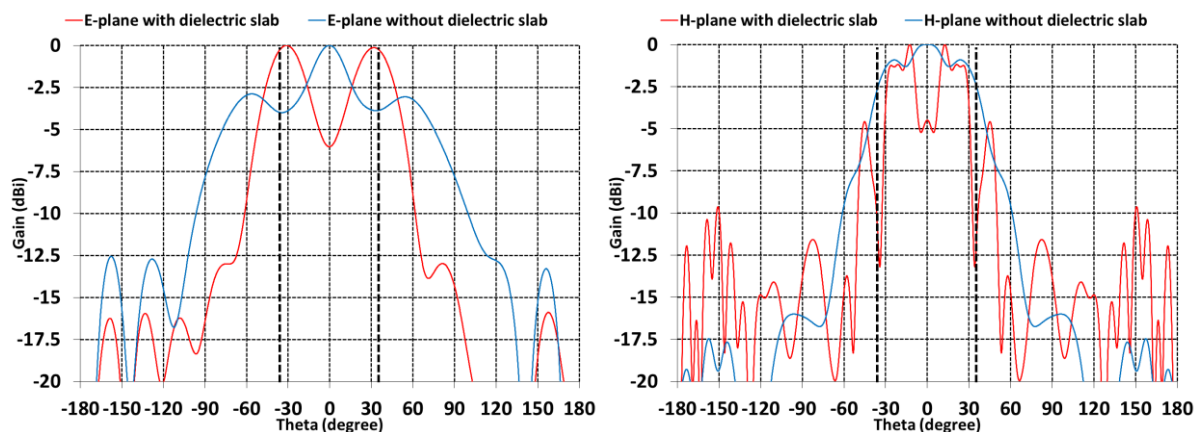
Figure 4-32: Normalized radiation patterns of a single ACMPP excited within a 9 \times 3 ACMPP elements array with and without a \lambda_0(5\text{mm}) dielectric slab at 60 GHz : (a) E-plane (b) H-plane.
