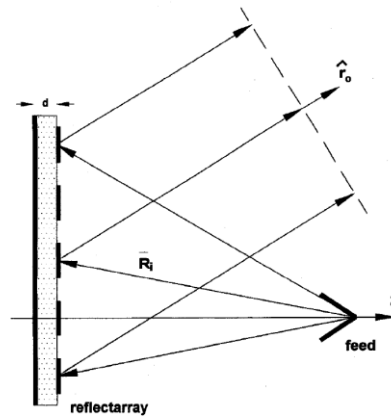
Figure 2-39: Geometry of the microstrip reflect-array [76].
