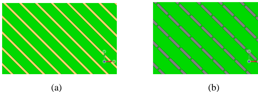
Figure 6-2: Twist-Reflector : (a) single Frequency (60GHz) (b) Dual-frequency (28 & 60 GHz).
