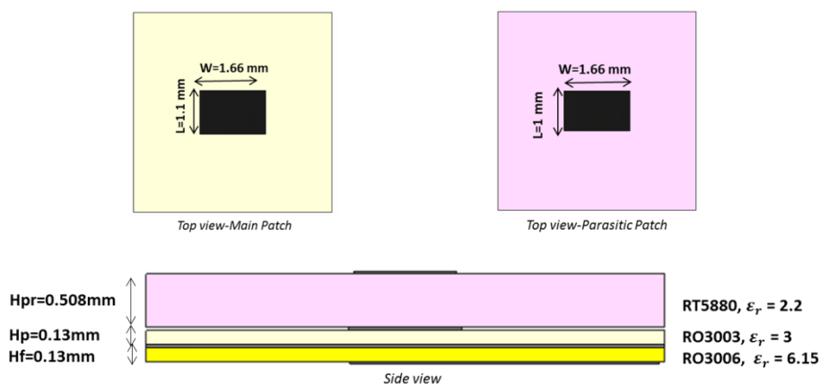
Figure 4-12: ACMPP with parasitic patch structure with design dimensions at 60 GHz.
