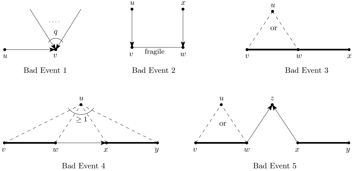
Figure 5.1: The five types of bad events in Algorithm 4. Bad edges are drawn in bold. (Note that possibly z = u in Bad Event 5.)
