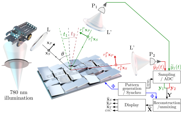
Fig. 1. Sketch of the 2-pixel CS polarimetric imaging setup proposed. It is inspired from the concept of SPC where the image is first spatially sampled by a DMD which reflects light in two directions, and where the total photon flux is detected on a single photodetector in each direction.
