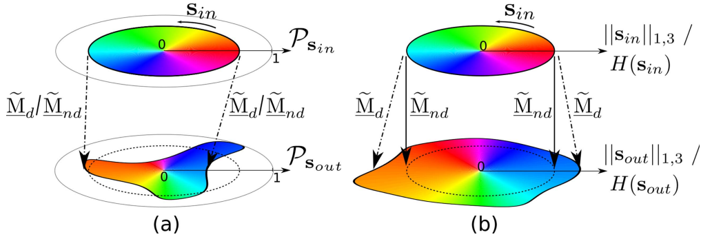
Figure 1. Schematic representation of the effect of a non-depolarizing ( \tilde{\mathbf{M}}_{nd} ) or a depolarizing ( \tilde{\mathbf{M}}_d ) transformation on (a) the standard DOP \mathcal{P} , and (b) the Minkowski metric \|\mathbf{s}\|_{1,3} or Shannon entropy H(\mathbf{s}) , for all possible input Stokes vectors \mathbf{s}_{in} (represented around a chromatic disk for the sake of simplicity).
