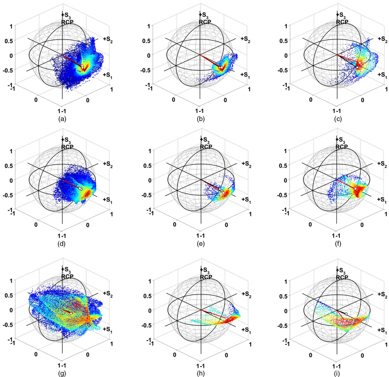
Fig. 11. (Color online) Repartition of the pixels SOP on Poincaré's sphere for a metallic sample (first line), a red paint sample (second line), and a green point sample (third line). First column, SOP in the whole ROI; second column, SOP in sub-ROI 1; third column, SOP in sub-ROI 2. Sub-ROIs are respectively defined in Figs. 9(b), 10(a), and 10(b).
