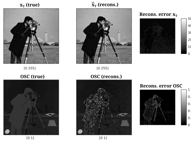
Figure 3.8: Example of numerical polarimetric imaging experiment. First row: total intensity image x_T , reconstruction \hat{x}_T and error map. Second row: true OSC image, reconstructed OSC image and error map.
