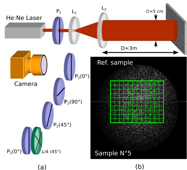
Fig. 1. (Color online) (a) Experimental setup, (b) example of an intensity image of the reference sample and sample 5 (green paint).
