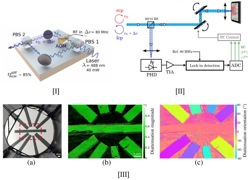
Figure 3.3: [I] Dual-frequency dual-polarization (DFDP) source based on a Mach-Zehnder architecture used for orthogonality breaking imaging at \lambda = 488 nm. [II] Sketch of the laser scanning imaging setup in reflection configuration. [III] Synthetic dichroic sample (made of polaroid sheets on a mirror) used for validation (intensity image). DSOB measurements results: linear diattenuation magnitude (b) and orientation (c) of the measured sample. Each image is 10 \times 7.5 mm.
