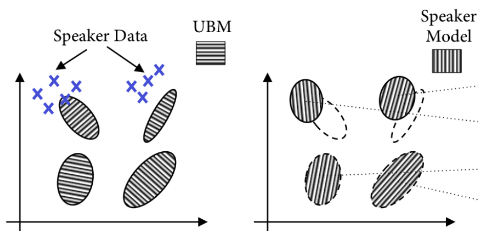
Figure 5.4: MAP adaptation procedure is illustrated for a 4 mixtures UBM. Source (Reynolds et al., 2000).
