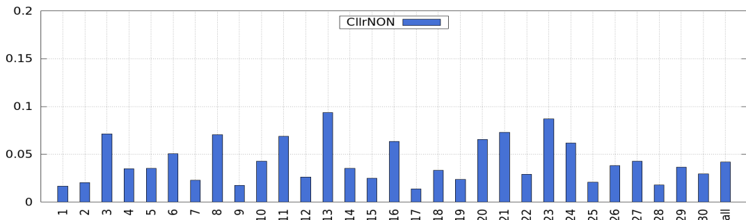
Figure 8.8: Bar-plot of C_{\text{llr}}^{\text{NON}} per speaker and for "all" (all speakers pooled together) extracted from 8.5.
