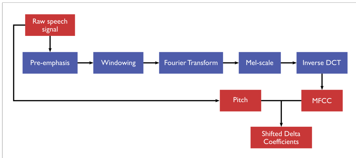
Figure 2.13: Pipeline for MFCC-SDC feature extraction.
