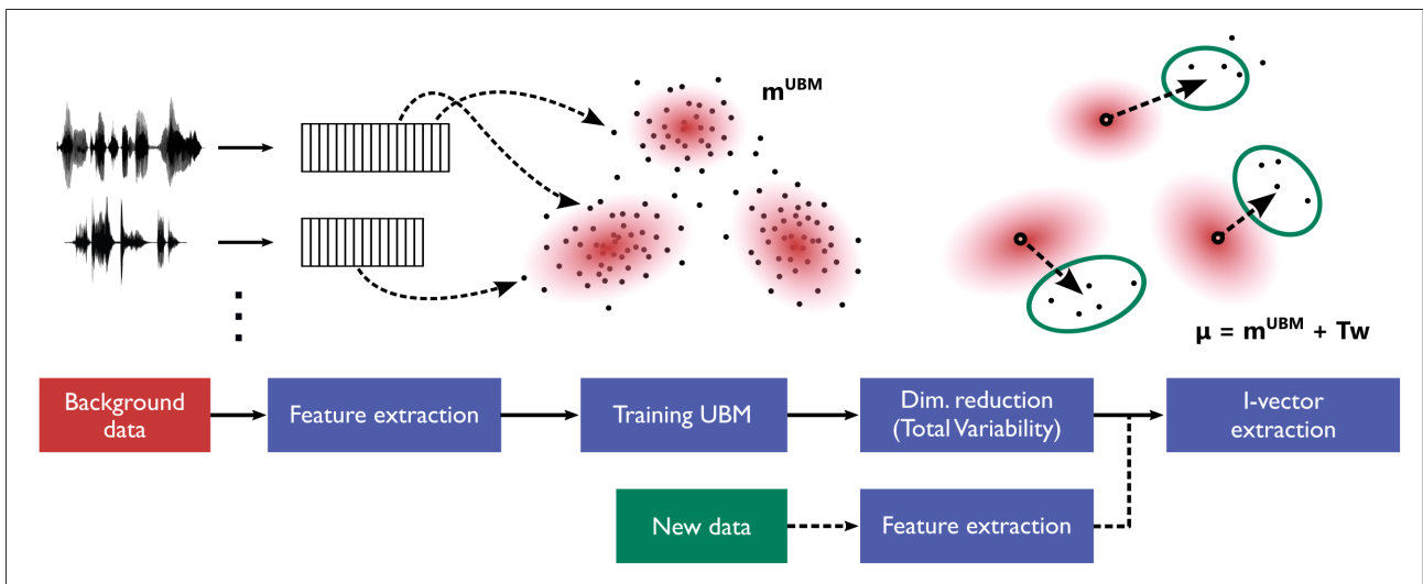
Figure 2.2: Pipeline for i-vector extraction.
