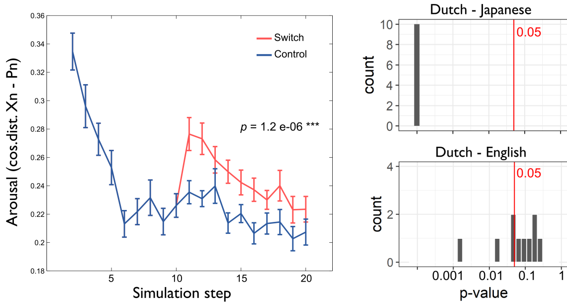
(a) Example of a simulated habituation experiment, using Dutch and Japanese samples.
