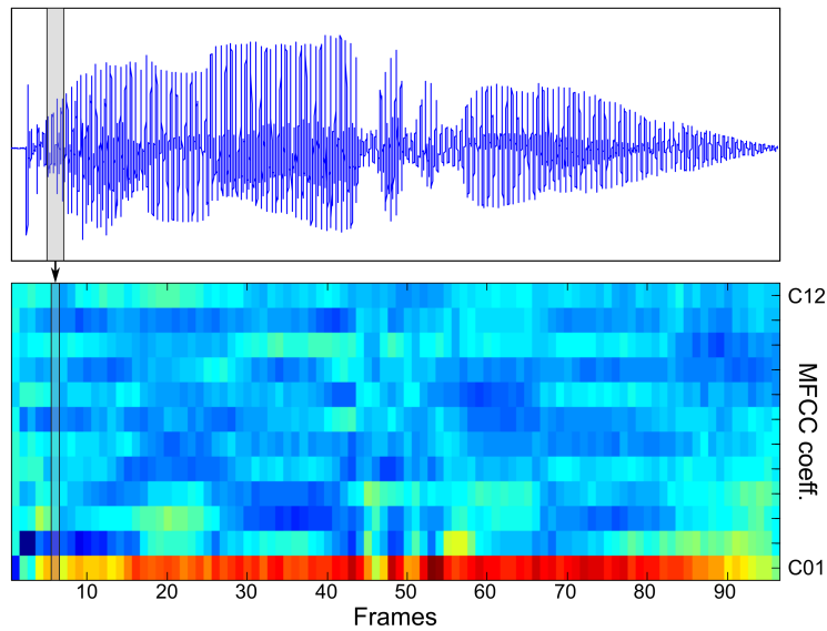
Figure 2.19: Speech signal (top) and magnitude of the first 12 Mel-Frequency Cepstral Coefficients at each time frame of the signal (bottom). Magnitude of the MFCCs is represented in a color scale.
