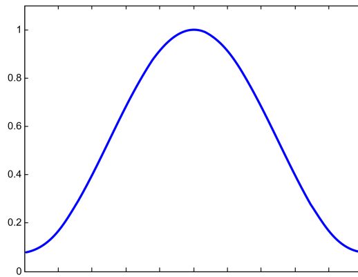
Figure 2.14: Hamming function.
