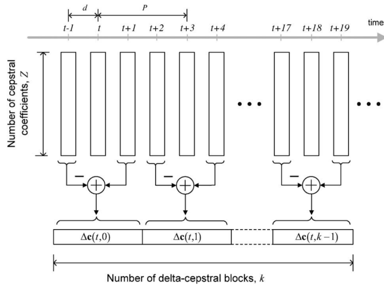
Figure 2.20: SDC feature extraction at frame time t . Reproduced from Li, Ma, and Lee, 2013.
