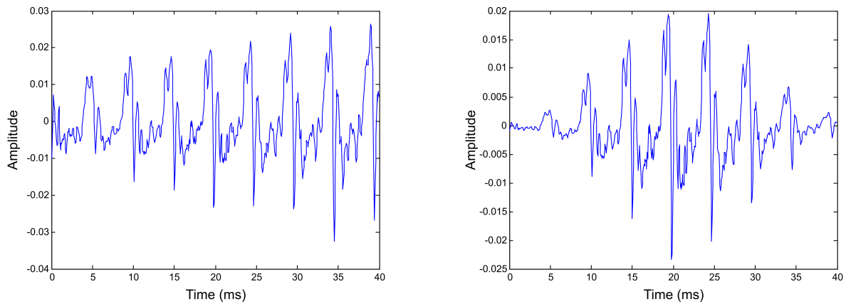
Figure 2.15: A 40 ms frame of the vowel [e] segmented from a Catalan utterance, before (left) and after (right) applying a Hamming window function.
