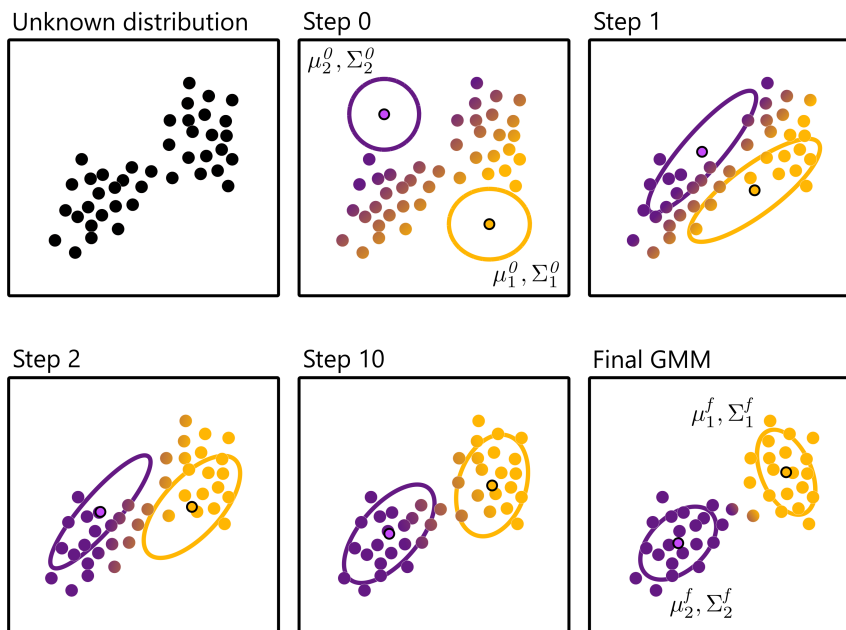
Figure 2.22: Illustrative example of the EM algorithm for estimation of parameters of a GMM with 2 Gaussian components.
