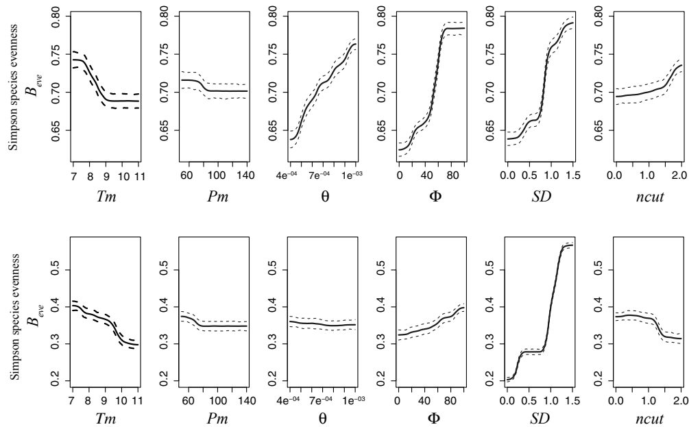
Figure III.9 – Main effects of six key parameters on Simpson species evenness B_{eve} , from dynamic trees performed on DYNAGRAM2 (A) and DYNAGRAM21 (B) outputs. Climate parameters: Tm (temperature), Pm (precipitation); soil fertility parameters: \Phi (fertiliser input), \theta (mineralization rate); defoliation parameters: SD (livestock density), ncut (mowing frequency).
