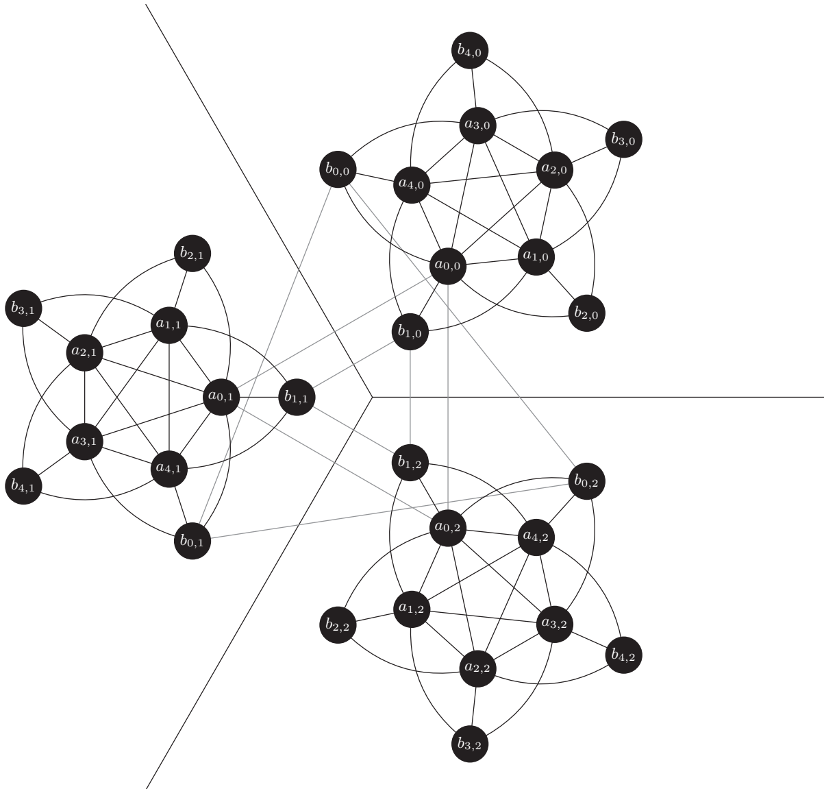
Figure 3.2.11: Example of a graph G_{n,k,l} = SF_{n,k} \square K_l for n = 5, k = 3, l = 3 .
