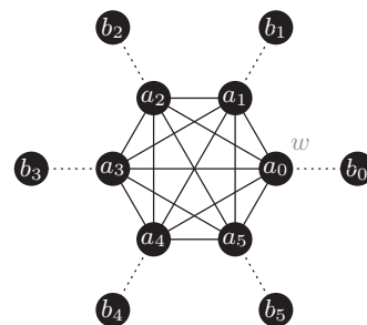
Figure 3.2.10: Tightness for \text{col}_X(G/e) = 2 + \text{col}_X(G) , for clarity we only drew the edges missing between A and B (dotted) except for a_0 and a_n in the first case, for which we show all of their edges.
