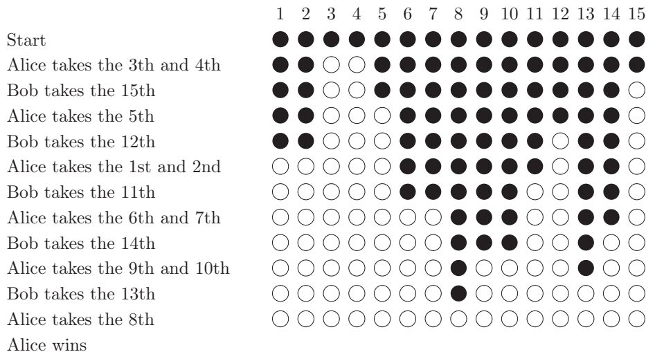
Figure 4.2.1: Example of game with 15 tokens initially.
