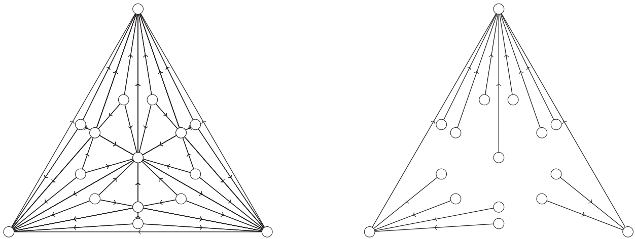
Figure 3.1.7: Example of k -tree with the orientation of \vec{G}_1 and the tree T of edges xf(x) .
