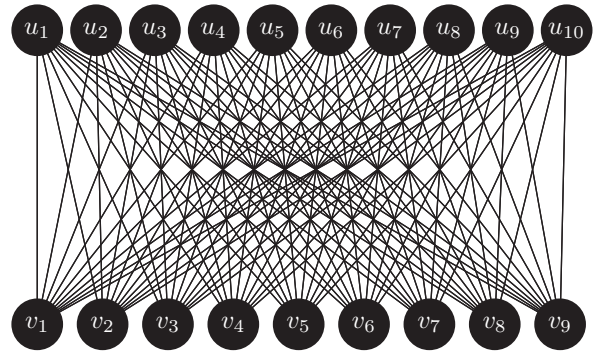
Figure 1.1.4: Example of a clique on 7 vertices and of a bipartite clique on 9 + 10 vertices.
