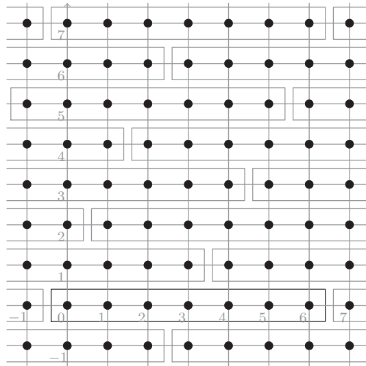
Figure 2.2.8: Example of C_7(1,3) in the square grid where the rectangles represent copies of C_7(1,3) . Remark that the neighborhood of (x,y) in the grid corresponds to the neighborhood of x+y \cdot d in the circulant graph.
