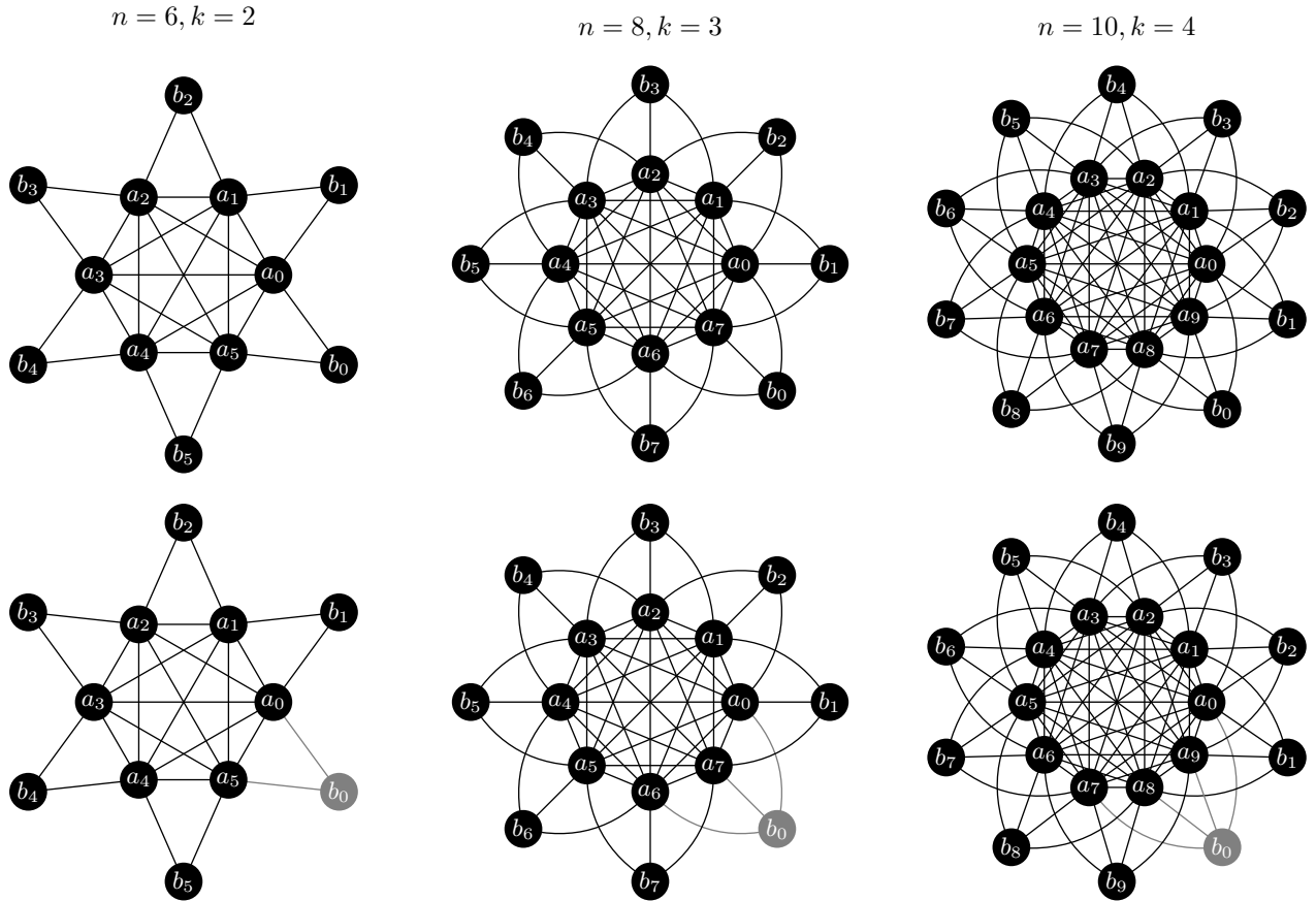
Figure 3.2.1: Examples of complete sunflowers SF_{n,k} and sunflowers missing a petal SF_{n,k}^*
